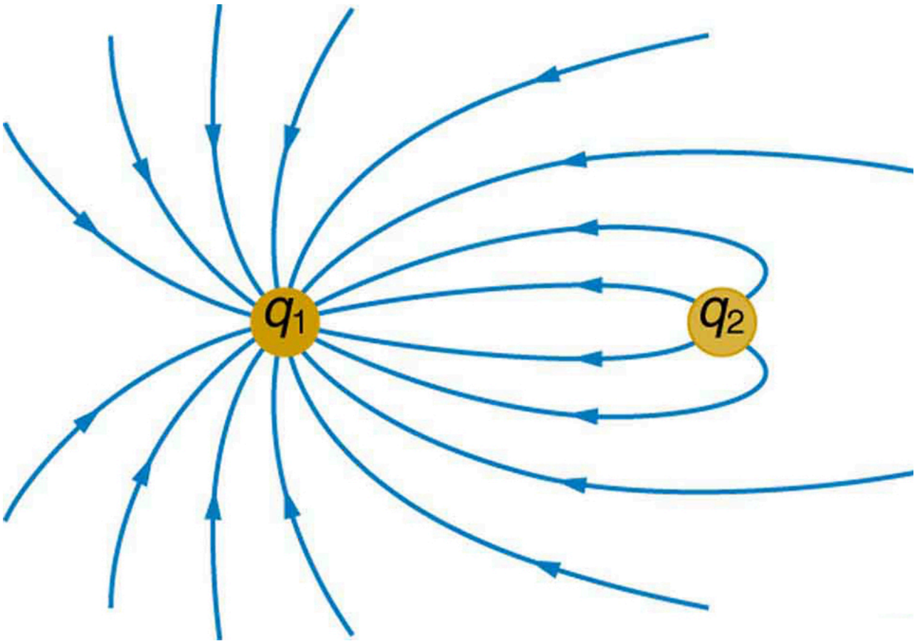
The electric field near two charges.
