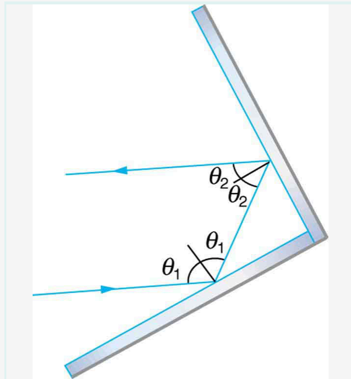
Figure 7: A corner reflector sends the reflected ray back in a direction parallel to the incident ray, independent of incoming direction.
