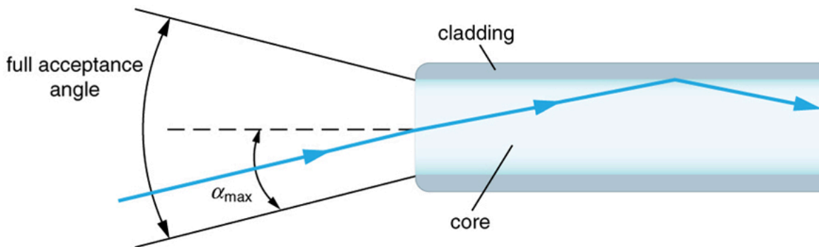
Light rays enter an optical fiber. The numerical aperture of the optical fiber can be determined by using the angle \alpha_{\max} .
