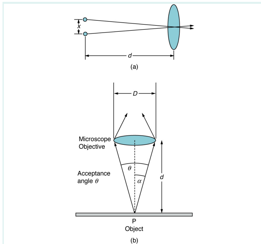
Figure 6: (a) Two points separated by a distance x and positioned a distance d away from the objective. (credit: Infopro, Wikimedia Commons) (b) Terms and symbols used in discussion of resolving power for a lens and an object at point P . (credit: Infopro, Wikimedia Commons)
