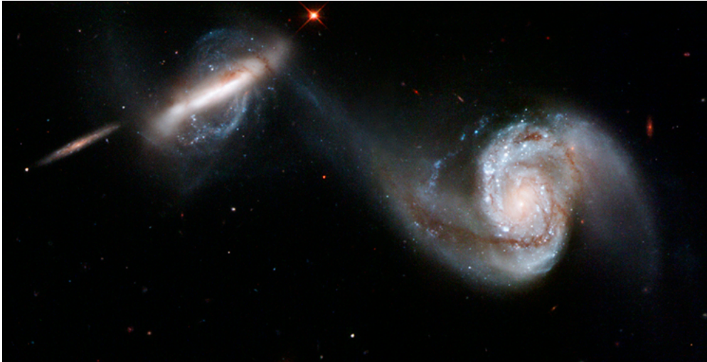
This NASA image of Arp 87 shows the result of a strong gravitational attraction between two galaxies. In contrast, at the subatomic level, the electrostatic attraction between two objects, such as an electron and a proton, is far greater than their mutual attraction due to gravity. (credit: NASA/HST)
