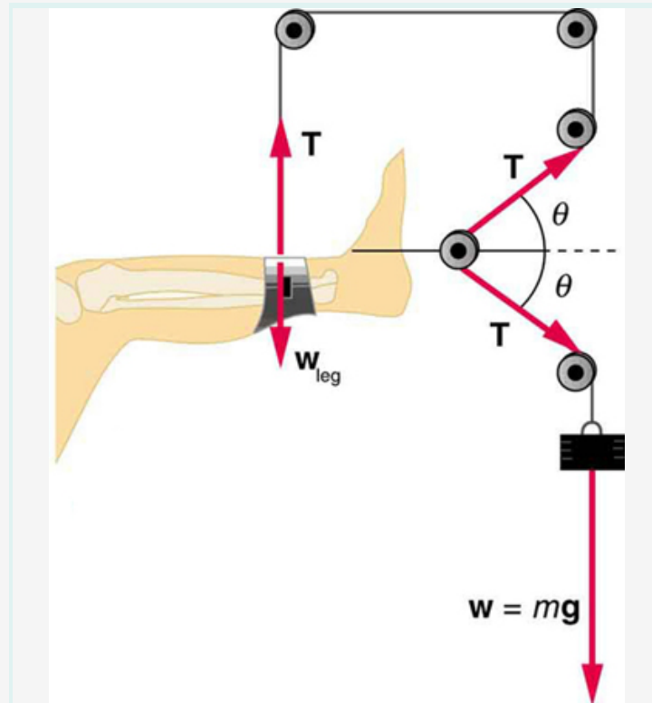
Figure 11: A leg is suspended by a traction system in which wires are used to transmit forces. Frictionless pulleys change the direction of the force T without changing its magnitude.
