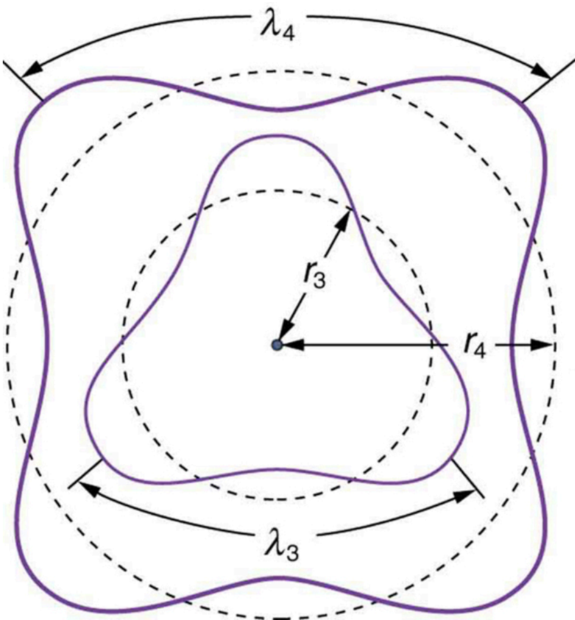
The third and fourth allowed circular orbits have three and four wavelengths, respectively, in their circumferences.
