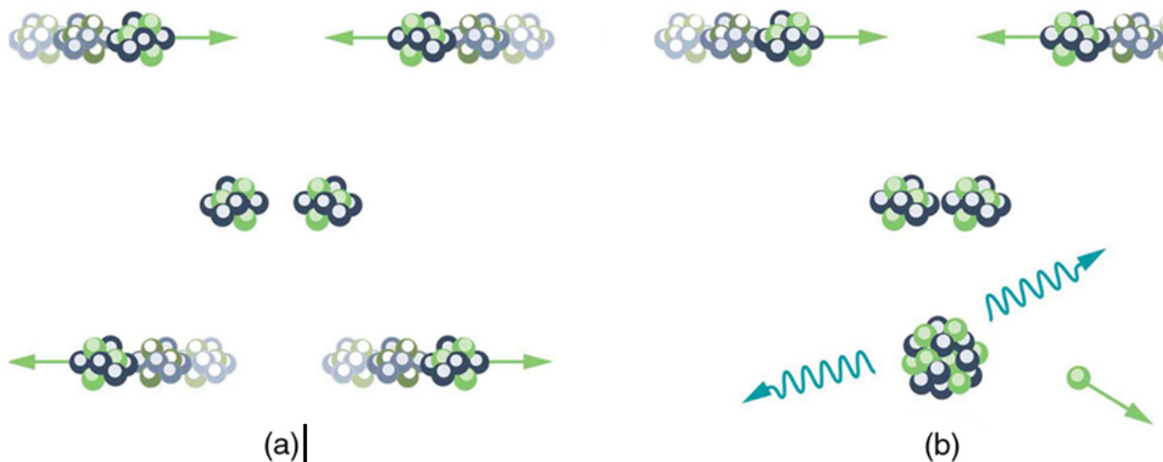
(a) Two nuclei heading toward each other slow down, then stop, and then fly away without touching or fusing. (b) At higher energies, the two nuclei approach close enough for fusion via tunneling. The probability of tunneling increases as they approach, but they do not have to touch for the reaction to occur.
