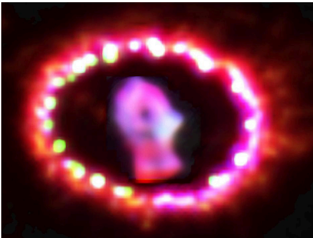
Supernovas are the source of elements heavier than iron. Energy released powers nucleosynthesis. Spectroscopic analysis of the ring of material ejected by Supernova 1987A observable in the southern hemisphere, shows evidence of heavy elements. The study of this supernova also provided indications that neutrinos might have mass. (credit: NASA, ESA, and P. Challis)
