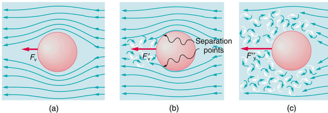
(a) Motion of this sphere to the right is equivalent to fluid flow to the left. Here the flow is laminar with (N^{\prime})_{\text{R}} less than 1. There is a force, called viscous drag (F_v) , to the left on the ball due to the fluid's viscosity. (b) At a higher speed, the flow becomes partially turbulent, creating a wake starting where the flow lines separate from the surface. Pressure in the wake is less than in front of the sphere, because fluid speed is less, creating a net force to the left (F'_v) that is significantly greater than for laminar flow. Here (N^{\prime})_{\text{R}} is greater than 10. (c) At much higher speeds, where (N^{\prime})_{\text{R}} is greater than (10^6) , flow becomes turbulent everywhere on the surface and behind the sphere. Drag increases dramatically.
