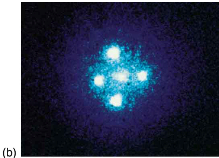
(a) Light from a distant galaxy can travel different paths to the Earth because it is bent around an intermediary galaxy by gravity. This produces several images of the more distant galaxy. (b) The images around the central galaxy are produced by gravitational lensing. Each image has the same spectrum and a larger red shift than the intermediary. (credit: NASA, ESA, and STScI)
