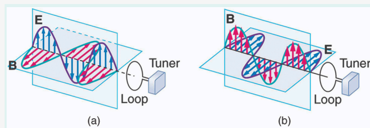
Figure 5: Electromagnetic waves approaching a wire loop.
