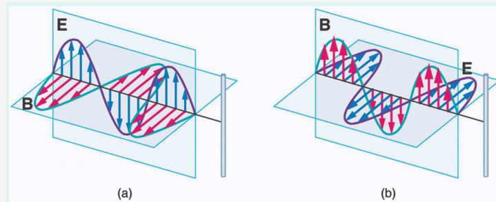
Figure 4: Electromagnetic waves approaching long straight wires.
