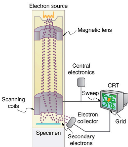
(a) Schematic of a scanning electron microscope (SEM) (a) used to observe small details, such as those seen in this image of a tooth of a Himipristis, a type of shark (b). (credit: Dallas Krentzel, Flickr)
