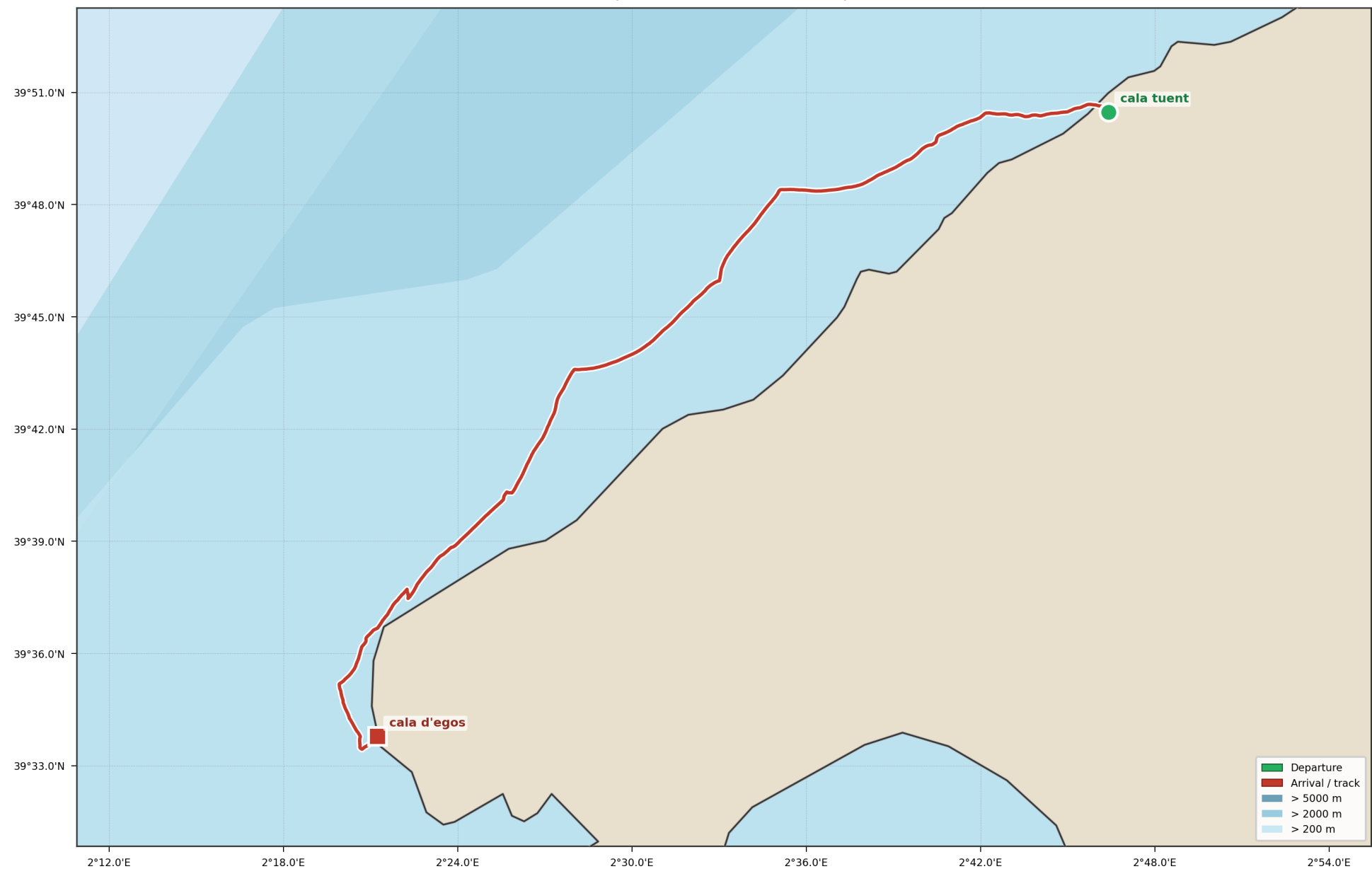
Track — ZOPA | cala tuent → cala d'egos | 30.0 nm nm
