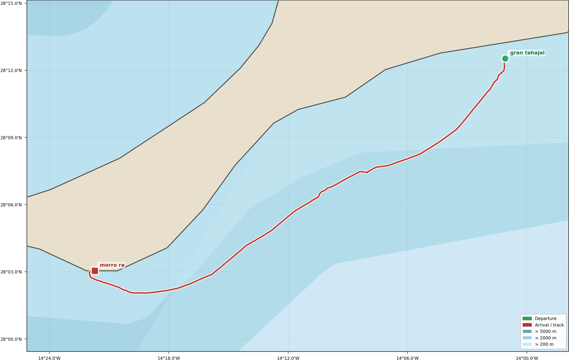
Track — ZOPA | gran tahajal → morro ra | 20.6 nm nm
