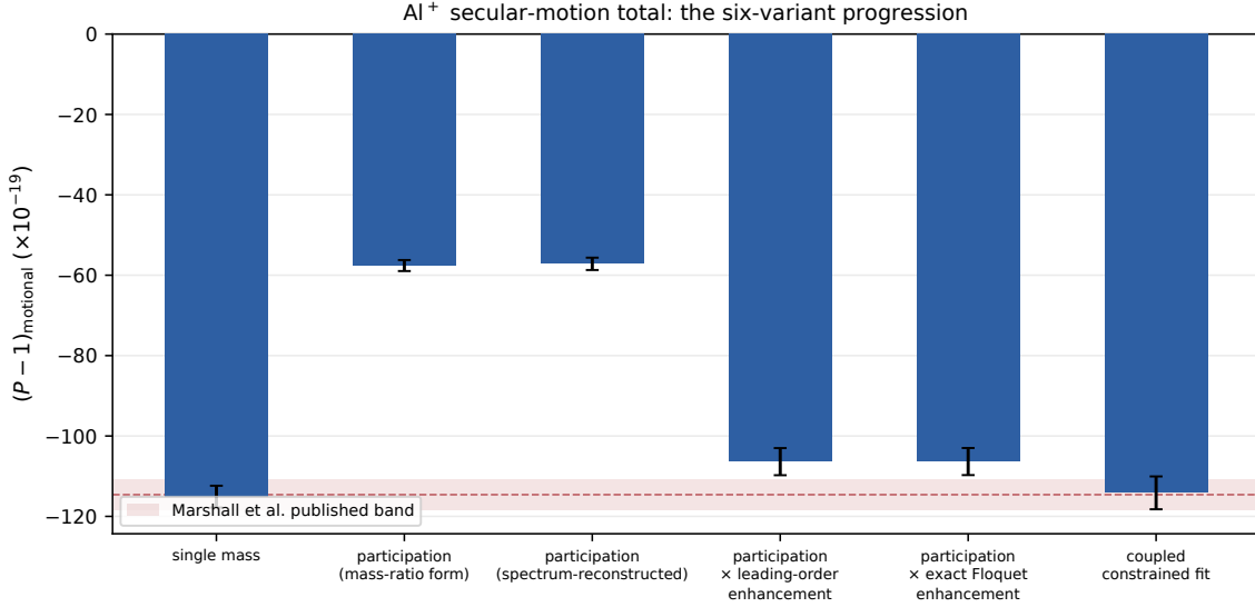
FIG. 5. The \text{Al}^+ secular-motion progression (Secs. IV H and IV I): six successive treatments of the same six-mode total, computed by the real engine against Marshall et al.’s published mode frequencies and occupations [22], plotted against Marshall et al.’s own published secular-motion band (shaded). The first variant carries one species mass through every mode. The second applies the two-ion participation factor from the \text{Al}^+/\text{Mg}^{25+} mass ratio alone (Wübbena et al. [17]). The third keeps that axial factor and reconstructs the radial pairs from the measured X/Y mode spectrum. The fourth multiplies the third’s participation by Berkeland’s leading-order mode-specific intrinsic-micromotion enhancement [18]. The fifth replaces that leading-order enhancement with the numerically exact Floquet solve of the same single-ion Mathieu equation. The sixth replaces the single-ion factorization entirely with the coupled two-ion Floquet solve’s constrained fit, this paper’s own headline treatment of the four radial modes. Error bars are each case’s own propagated 1-sigma uncertainty. Regenerated by paper/figures/fig8_motional_progression.py against the real benchmarks/run_motional_al_ion.py case objects.
