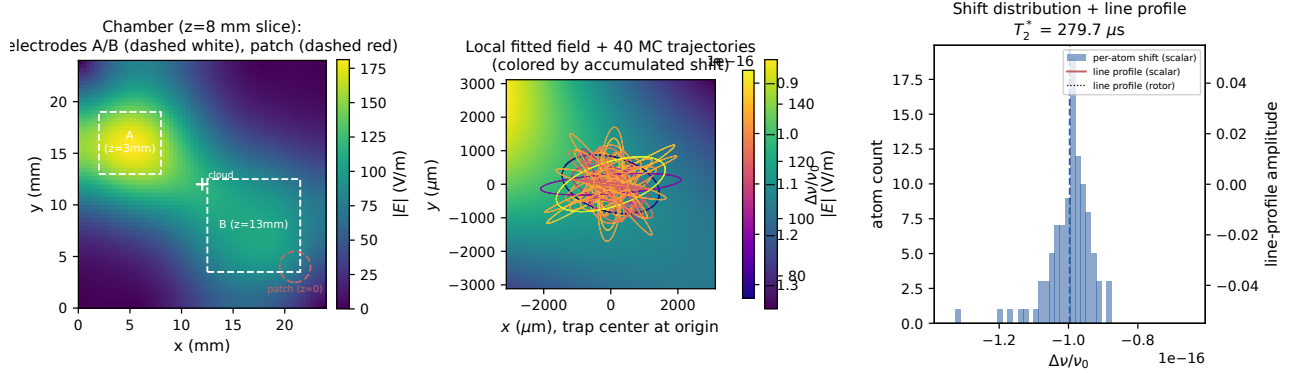
FIG. 5. The showcase scenario (Sec. V). (a) Whole-chamber field magnitude at the trap’s z -plane, with the two asymmetric electrodes and the patch-potential wall spot marked (dashed outlines, projected onto this plane; see the electrode/patch z -positions annotated on the panel). (b) The locally fitted field (the same FieldSmoother fit the pipeline evaluates) with a subsample of Monte Carlo trajectories overlaid, each colored by its final accumulated fractional shift. (c) The per-atom shift distribution (histogram) and the resulting spectral line profile (both trajectory- and rotor-mode evaluations overlaid), with T_2^* annotated. Regenerated by paper/figures/fig4.showcase_gradient_dispersion.py against the real pipeline, using examples/showcase_gradient_dispersion_sr87.yaml and its generating field examples/showcase_field.txt ( examples/generate_showcase_field.py ).
