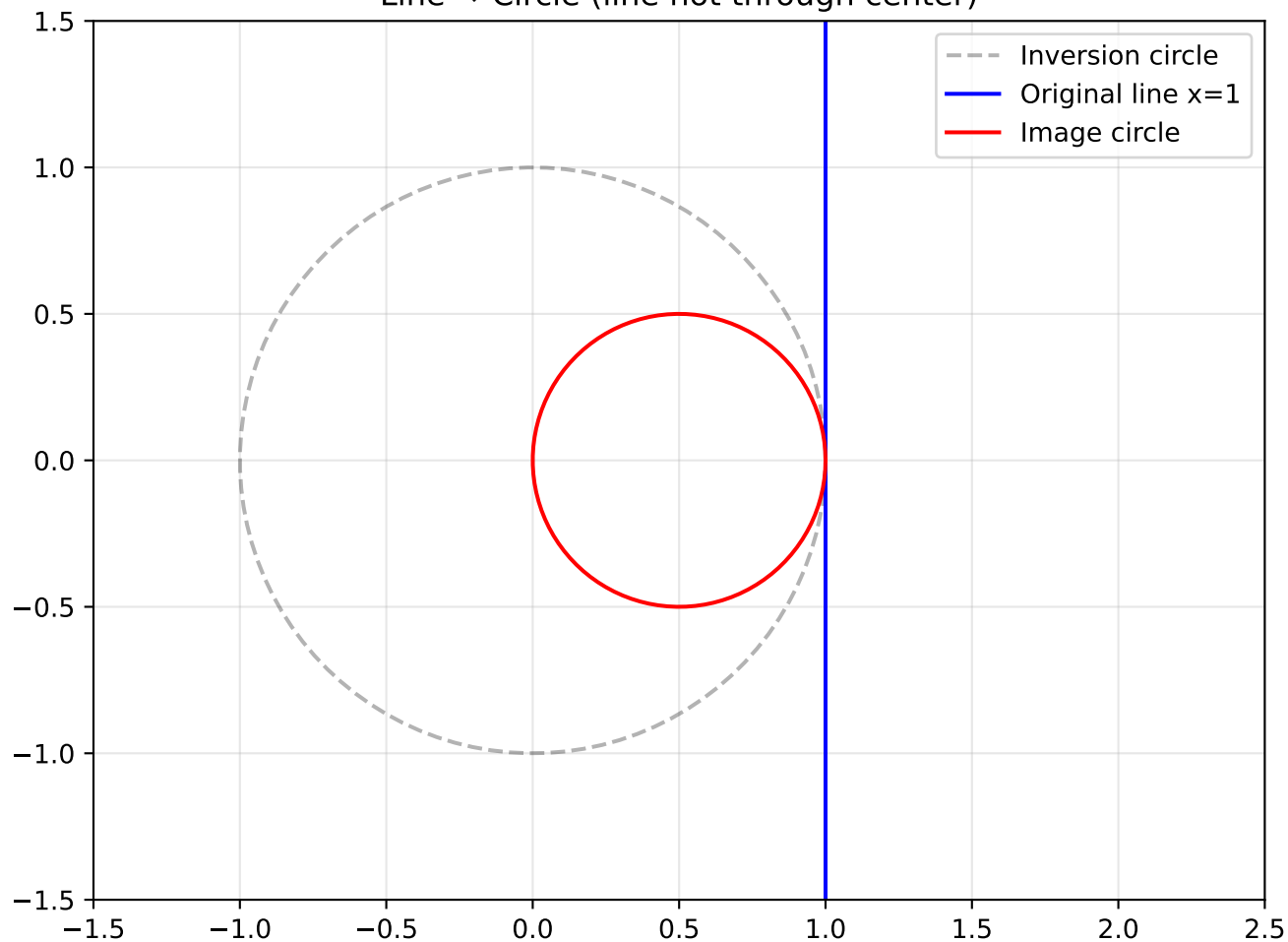
Line \rightarrow Circle (line not through center)
