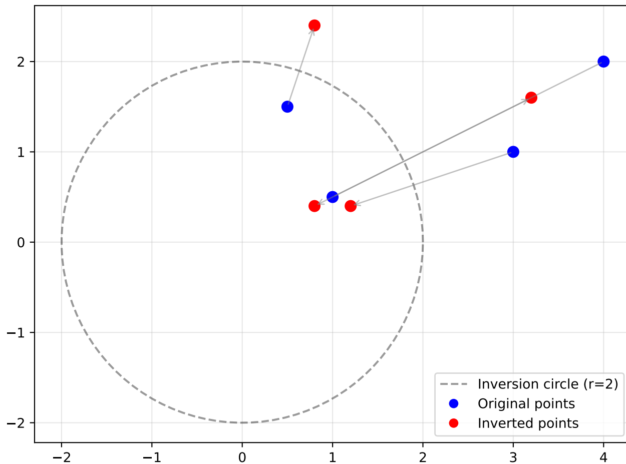
Point inversion in a circle
