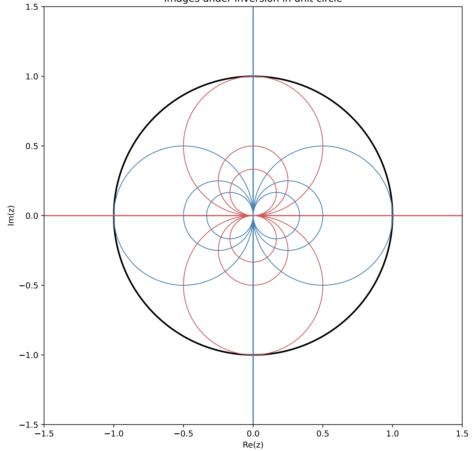
Images under inversion in unit circle
