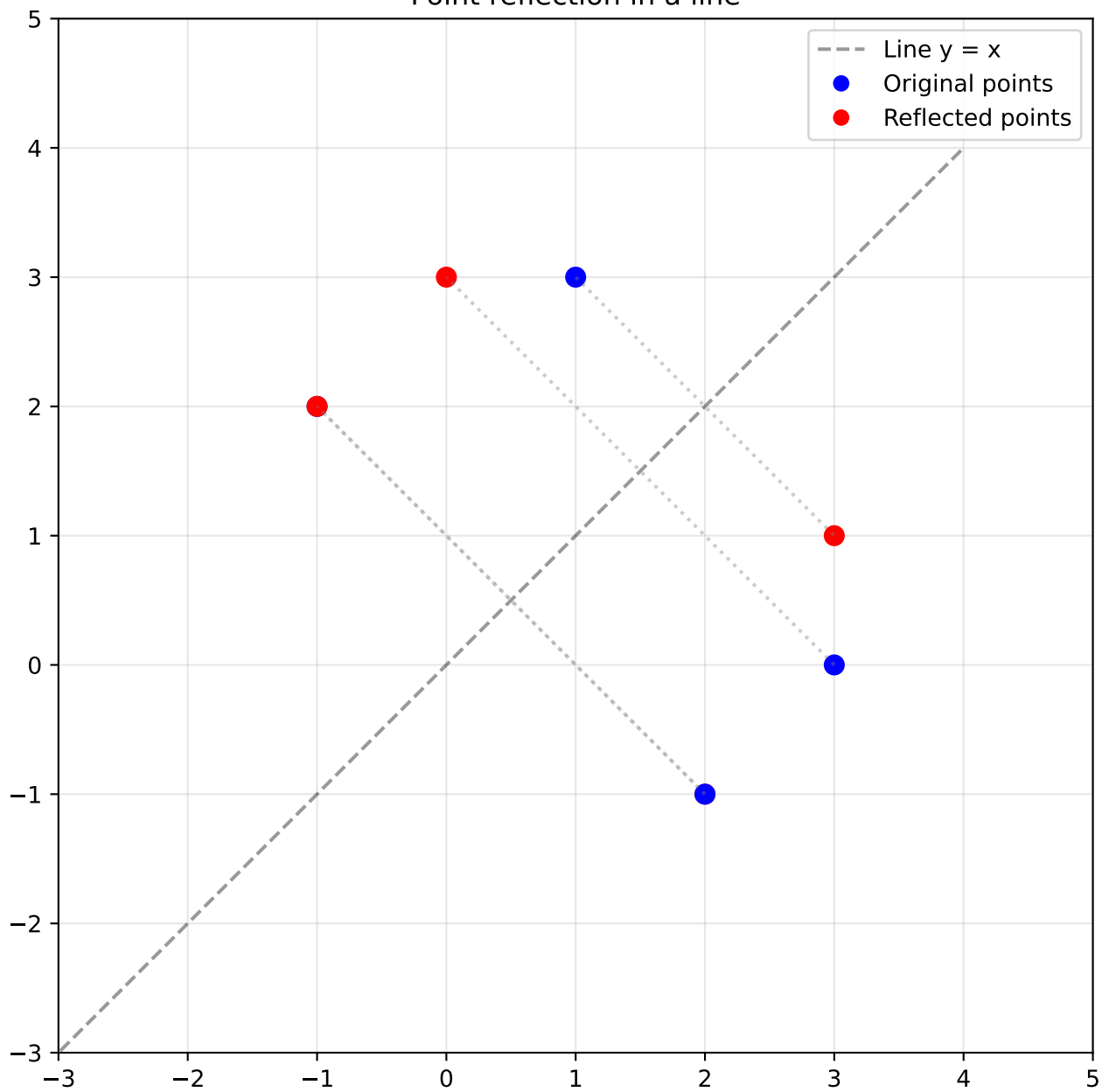
Point reflection in a line
