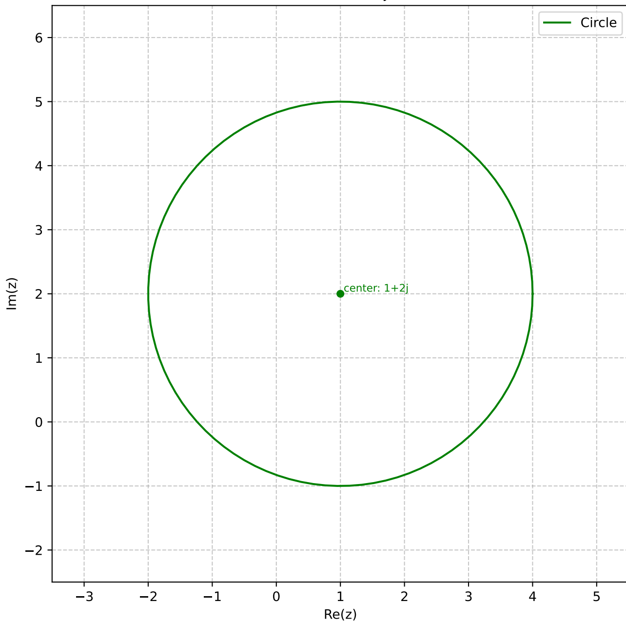
Circle with Center at 1+2j and Radius 3
