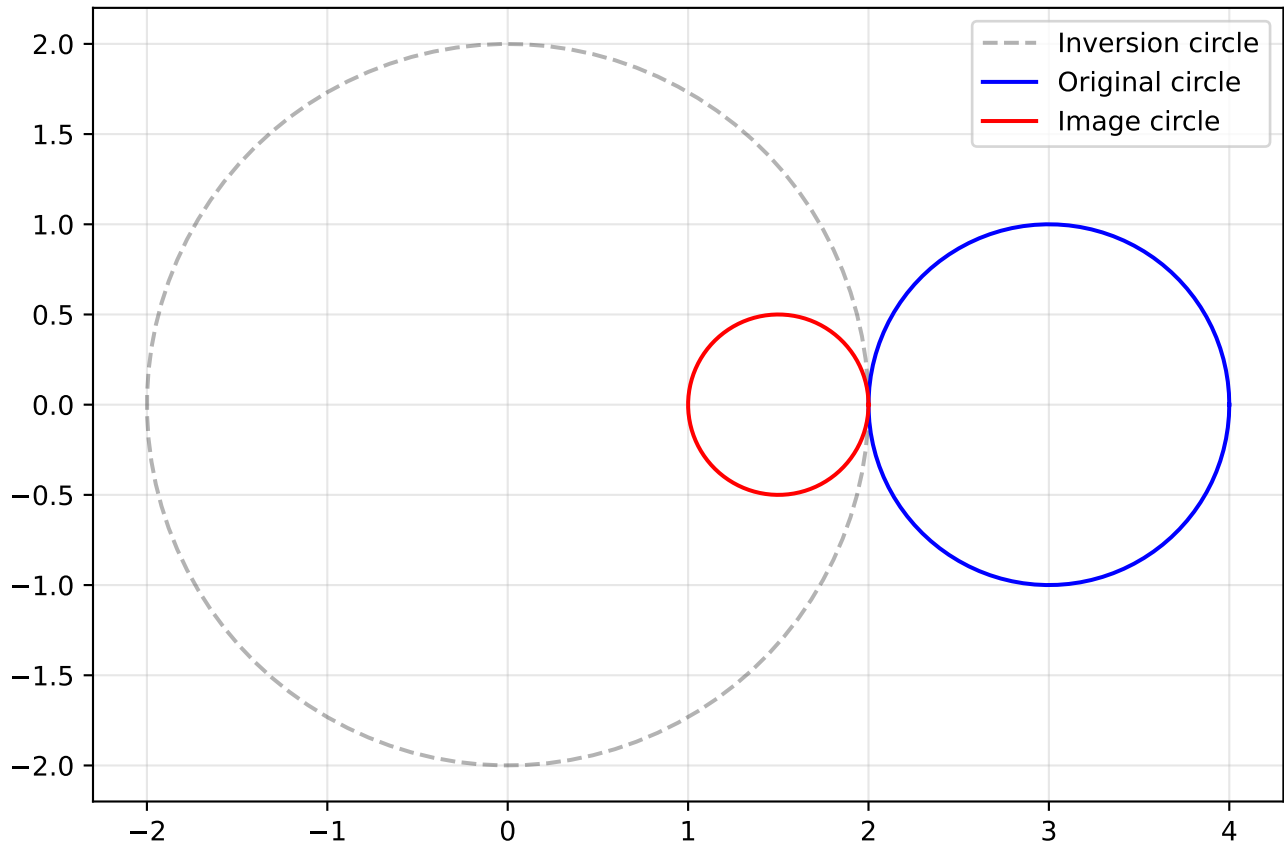
Circle \rightarrow Circle (not through center)
