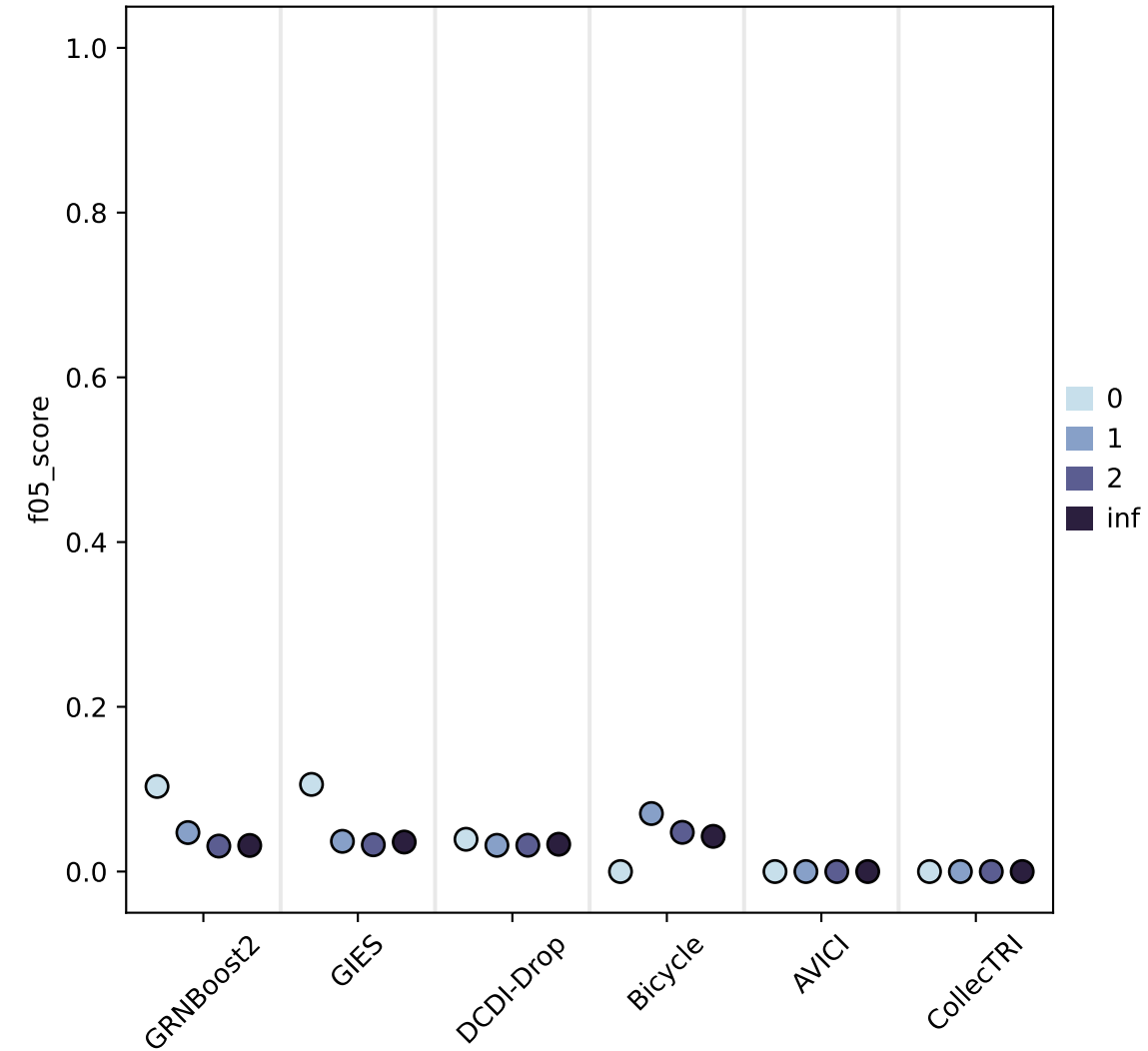
f05_score over different number of indirect edges added
