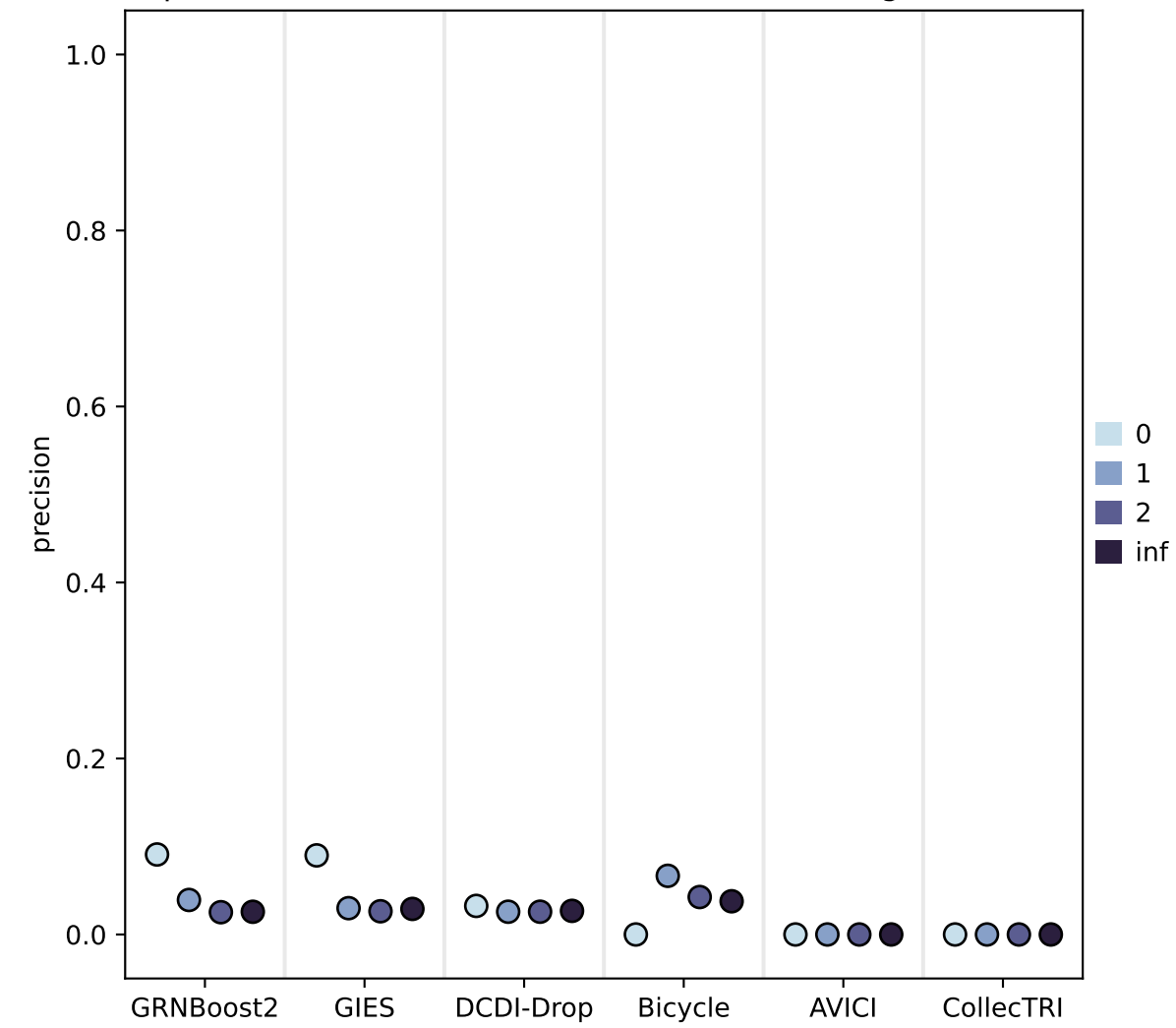
precision over different number of indirect edges added
