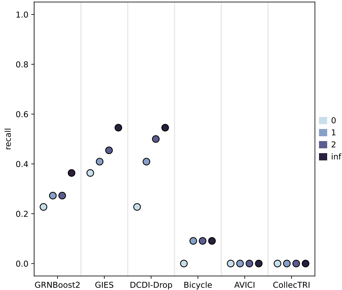
recall over different number of indirect edges added
