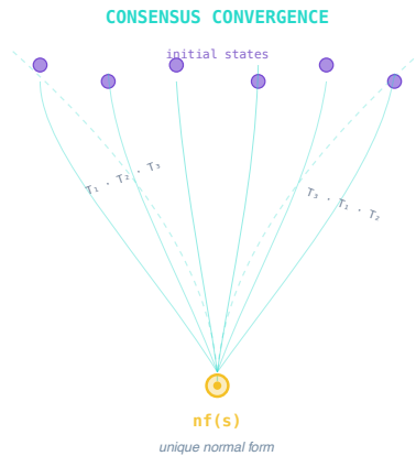
Figure 1.1: Many local descriptions for a fixed boundary problem can be repaired in different orders, yet converge to one shared normal form when the overlap rules satisfy the transactional confluence conditions.
