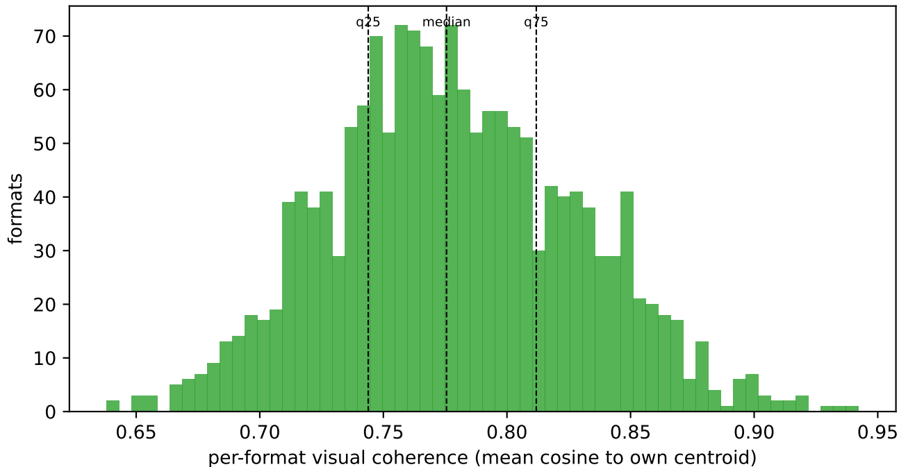
Visual coherence distribution (n=1622)
