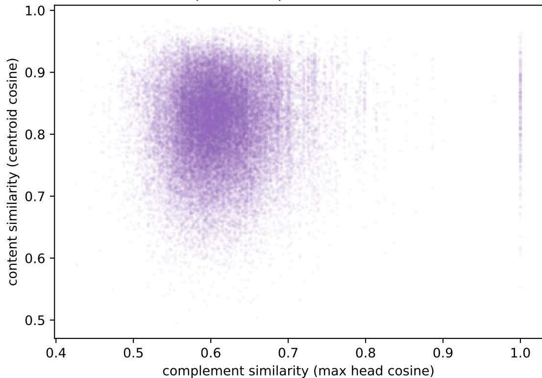
EXPRESS within-pairs: complement vs content ( \rho=0.041 )
