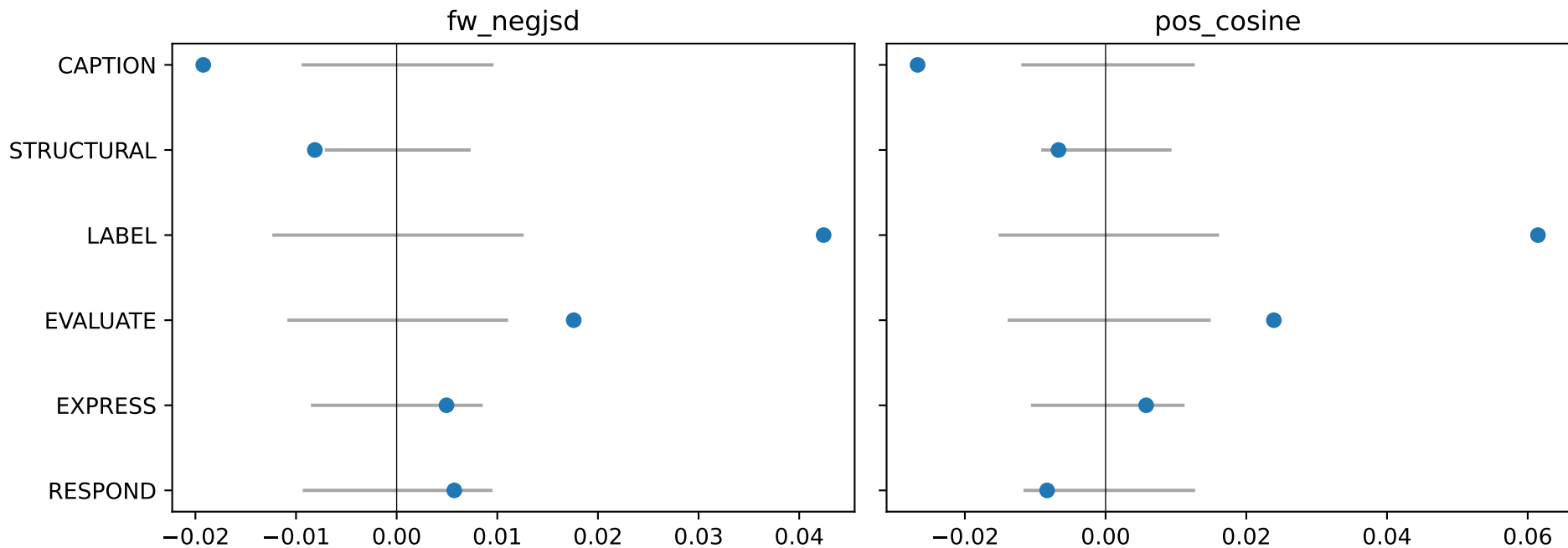
Per-family one-vs-rest effects (dots) vs permutation null 95% bands (grey)
