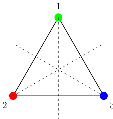
FIGURE 1.2. Symmetries of the triangle.
