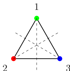
FIGURE 1.2. Symmetries of the triangle.
