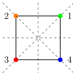
FIGURE 1.4. The symmetries of the square.
