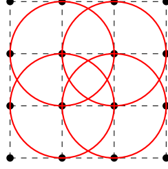
FIGURE 10.1. \mathbb{C} is covered by open unit disks of radius one and centers in \mathbb{Z}[i] .
