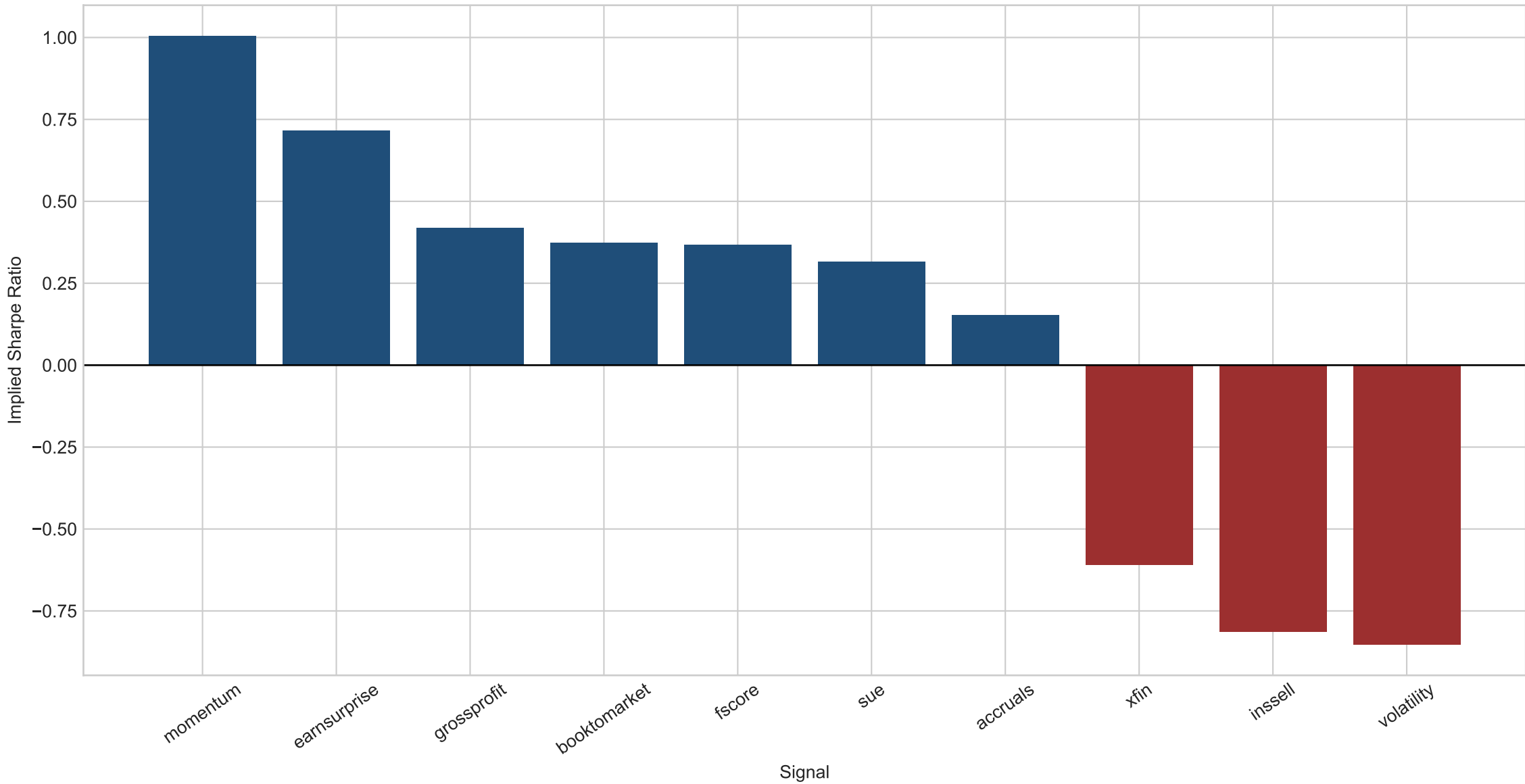
Step C: Implied Sharpe Ratios from Step B t-Statistics
