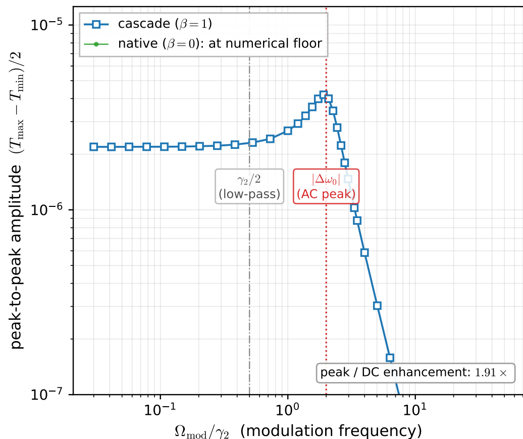
(b) Modulator transfer function
