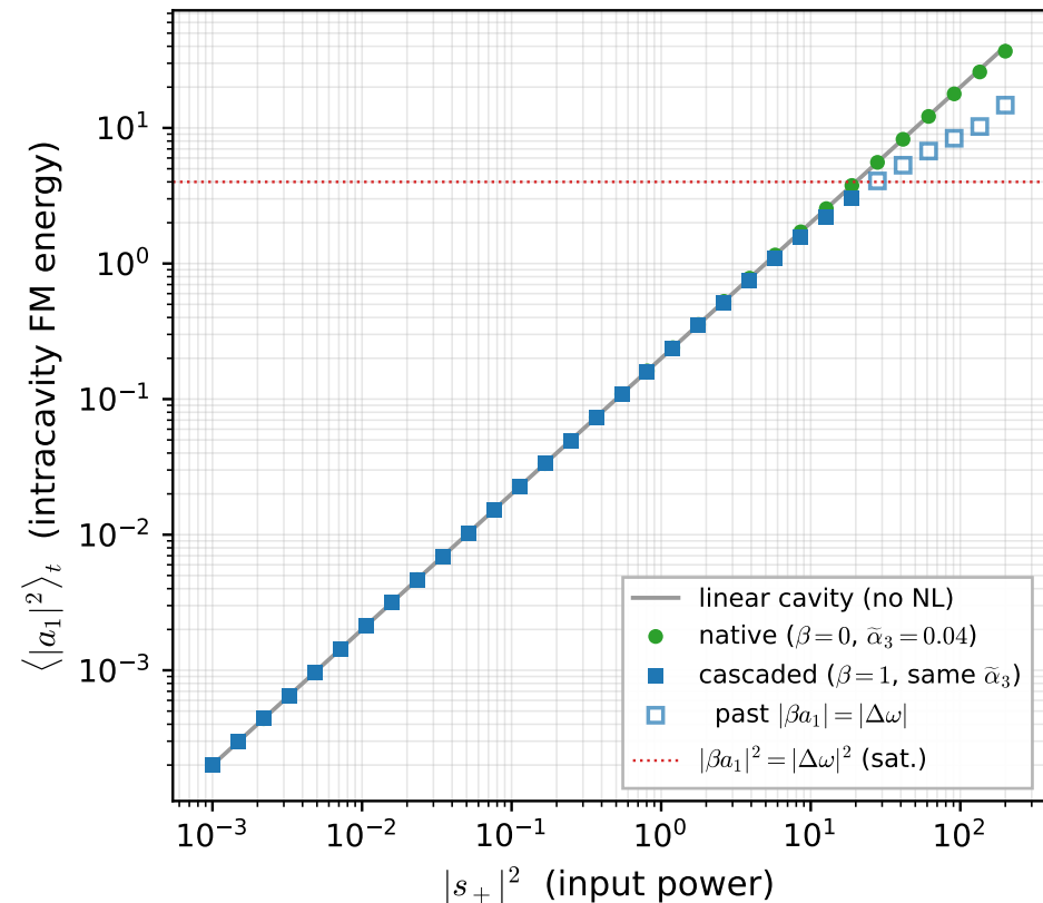
(a) FM energy: same input, same FM cavity
