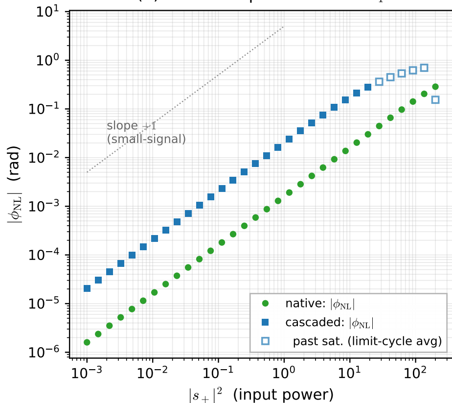
(b) Nonlinear phase shift on a_1
