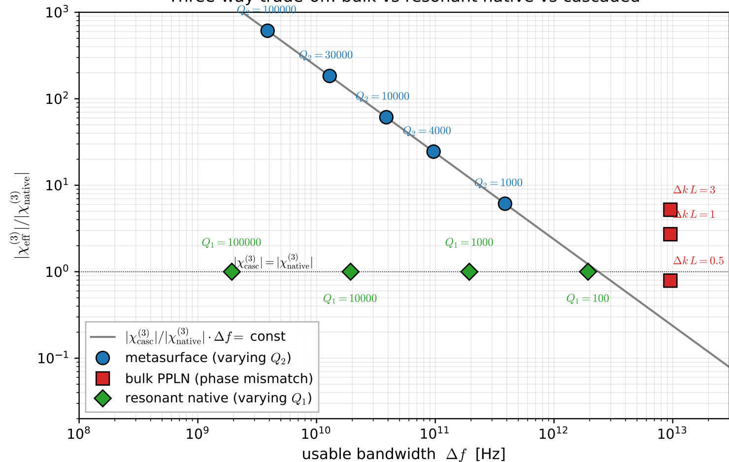
Three-way trade-off: bulk vs resonant native vs cascaded
