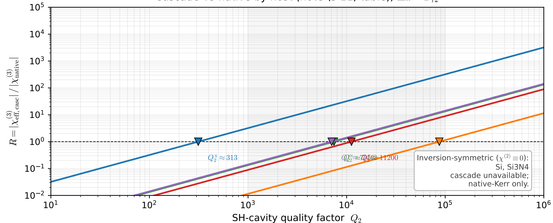
Cascade-vs-native by host (note \S 11, table); \Delta\omega = 2\gamma_2
