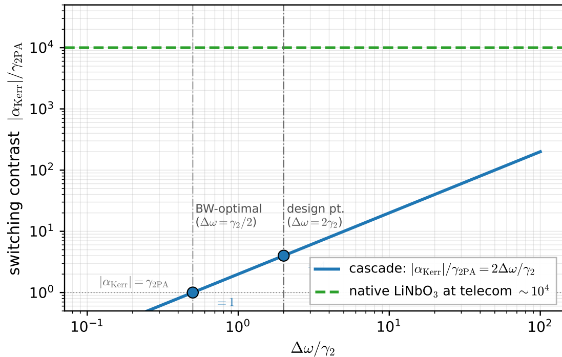
(b) Cascade is contrast-limited; native is essentially lossless
