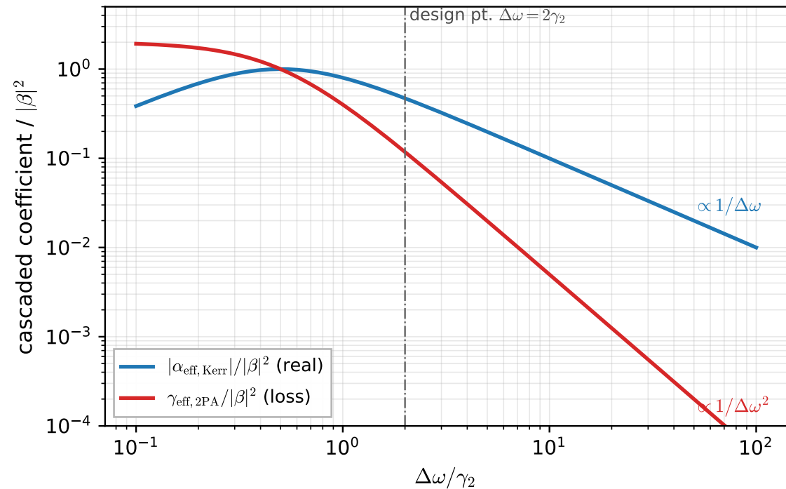
(a) Kerr falls as 1/\Delta\omega ; TPA falls faster, as 1/\Delta\omega^2
