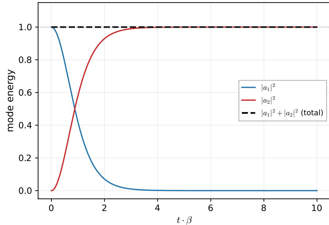
(a) Correct DFG coupling — total energy conserved
