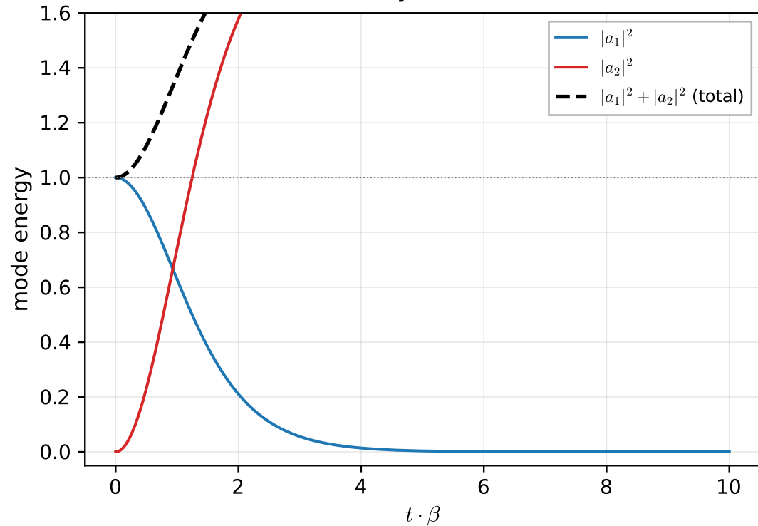
(b) DFG halved — Manley–Rowe violated, total drifts
