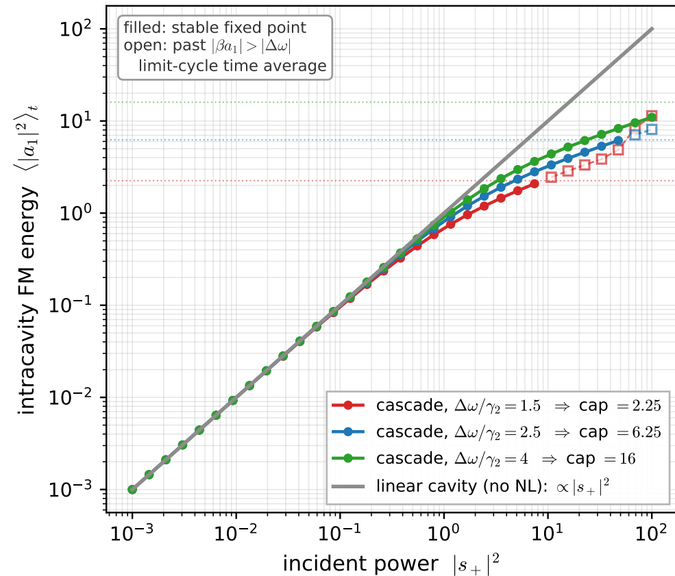
(a) Cascade clamps |a_1|^2 ; cap tunable via \Delta\omega
