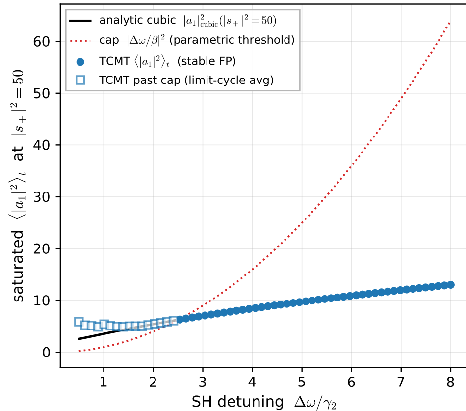
(b) Saturated FM energy vs \Delta\omega at high pump
