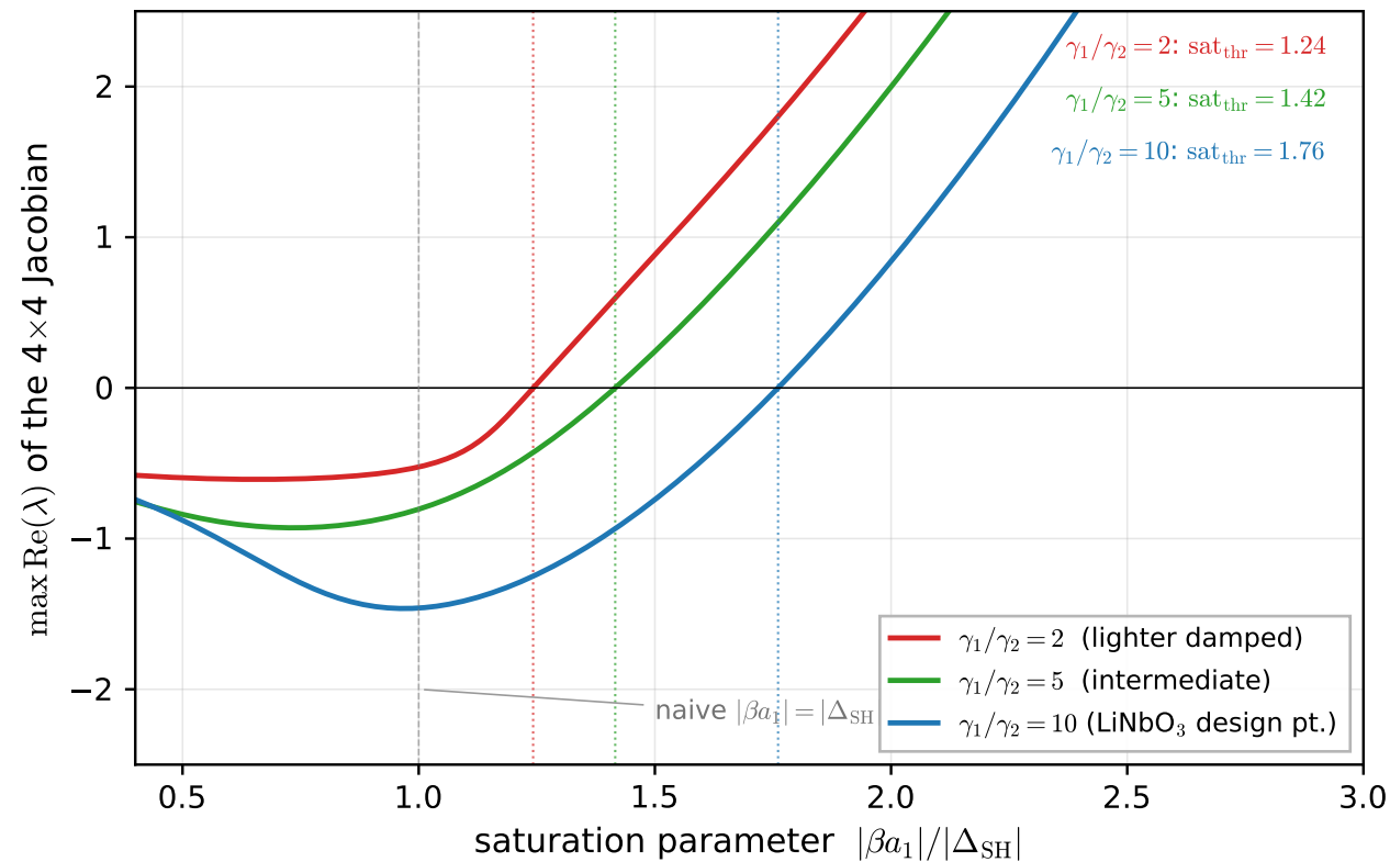
(a) Linear-stability threshold vs FM damping
