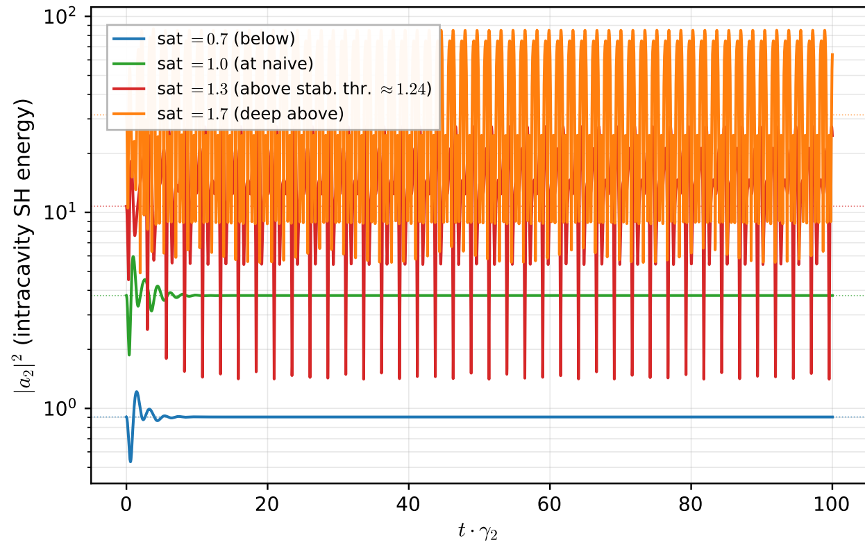
(b) Time-domain validation, \gamma_1/\gamma_2 = 2
