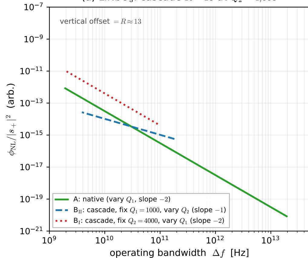
(a) \text{LiNbO}_3 : cascade R \simeq 13 at Q_2 = 4,000
