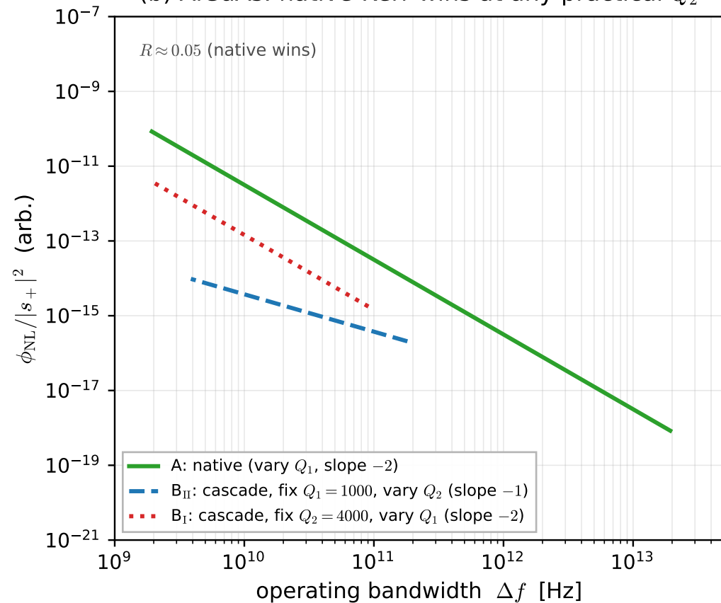
(b) \text{AlGaAs} : native-Kerr wins at any practical Q_2
