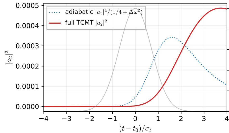
(c) Bandwidth limit (time-domain sum rule)
