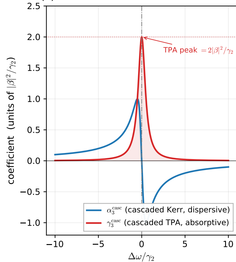
(a) Cascade coefficients vs SH detuning
