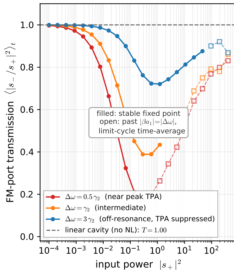
(b) Intensity-dependent transmission (full TCMT)
