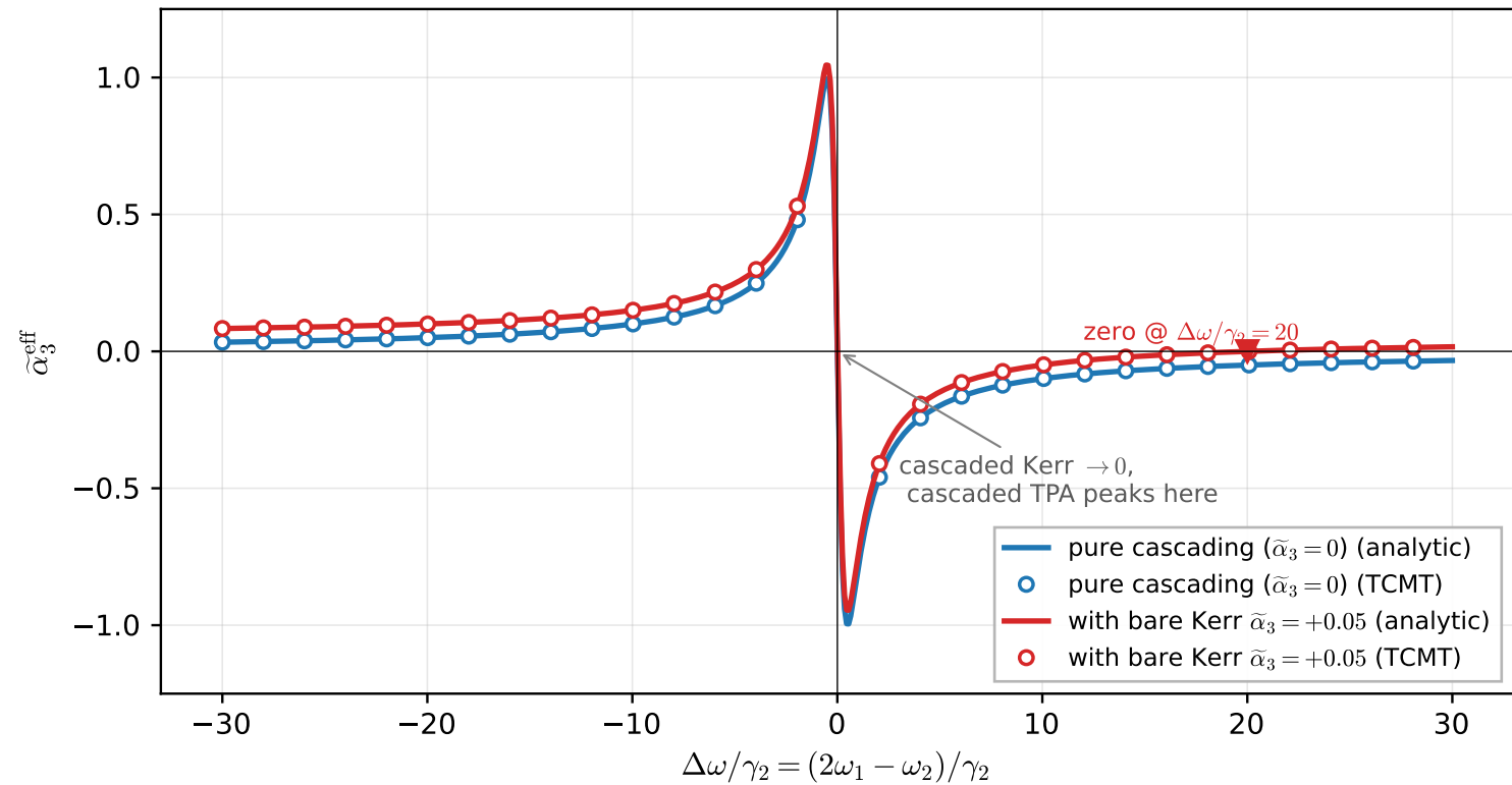
Sign tunability: walking the SH resonance through twice the FM
