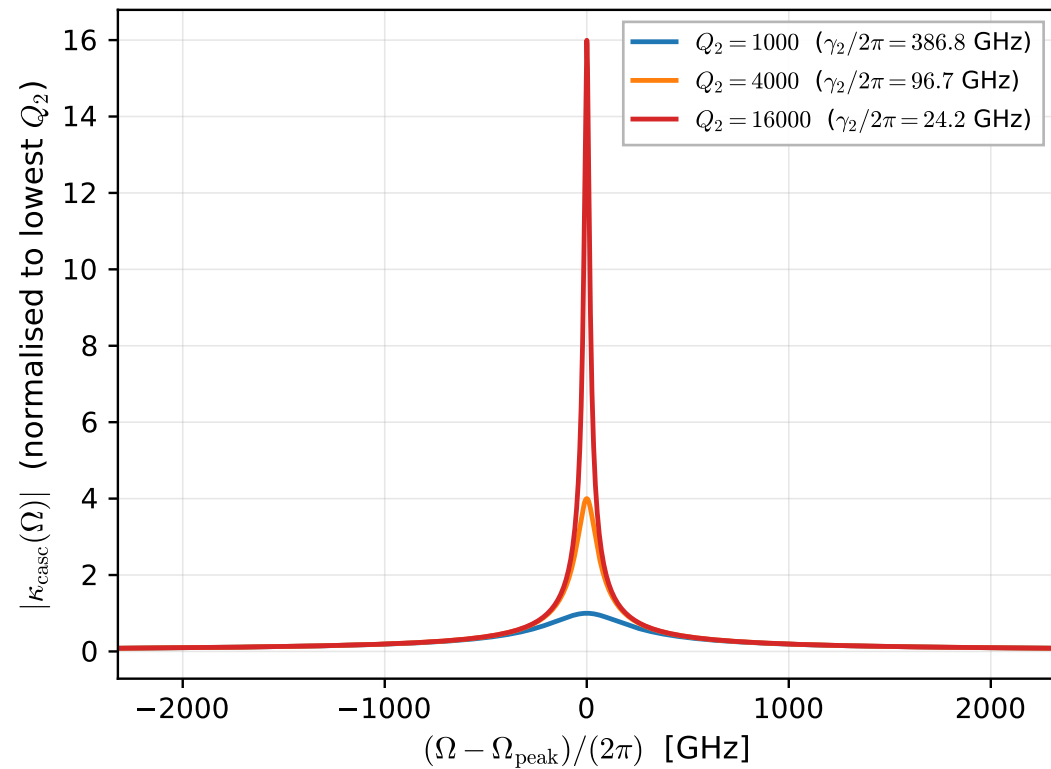
(a) Frequency response — peaks aligned
