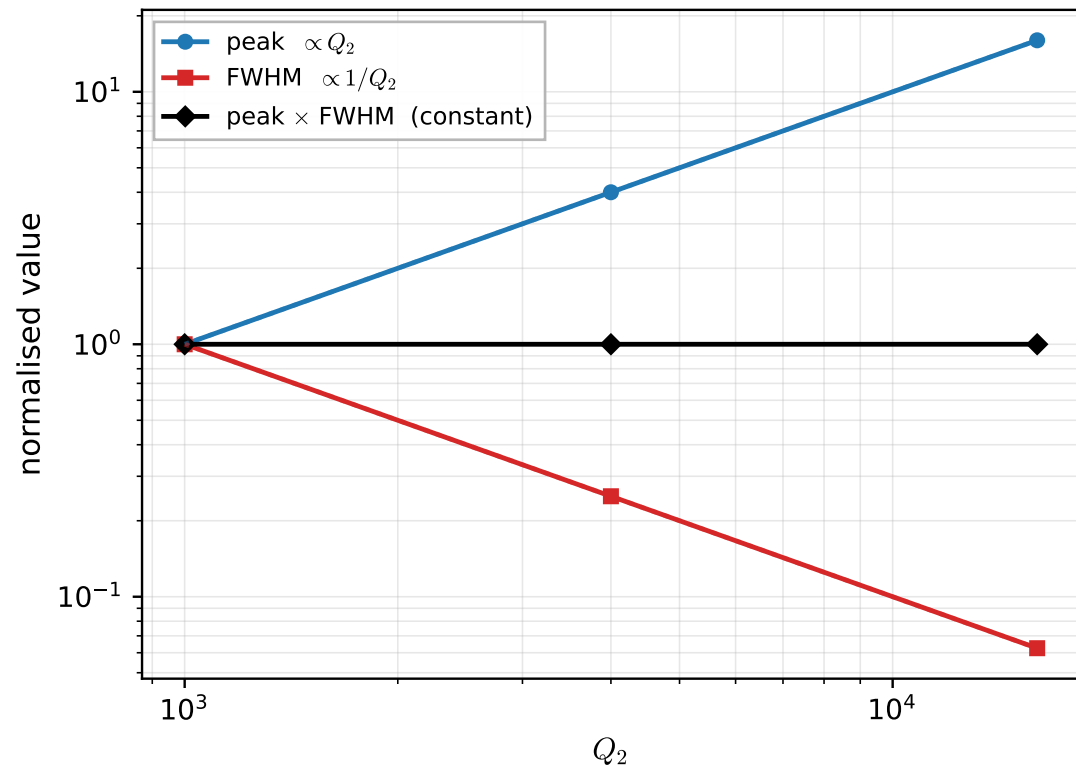
(b) Bandwidth-enhancement sum rule
