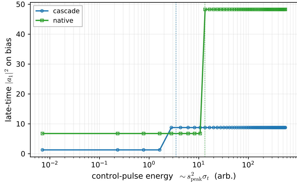
(b) Threshold sweep: cascade switches at much lower energy
