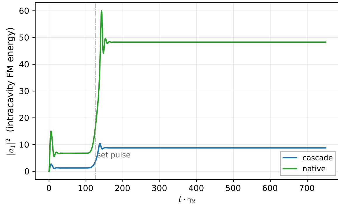
(a) Switching events at minimum control-pulse energy
