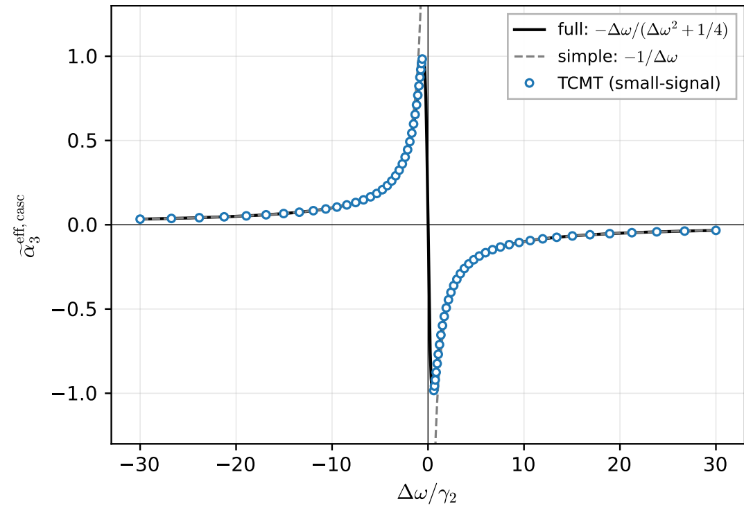
(a) Cascaded Kerr (real part) — sign-tunable through \Delta\omega=0
