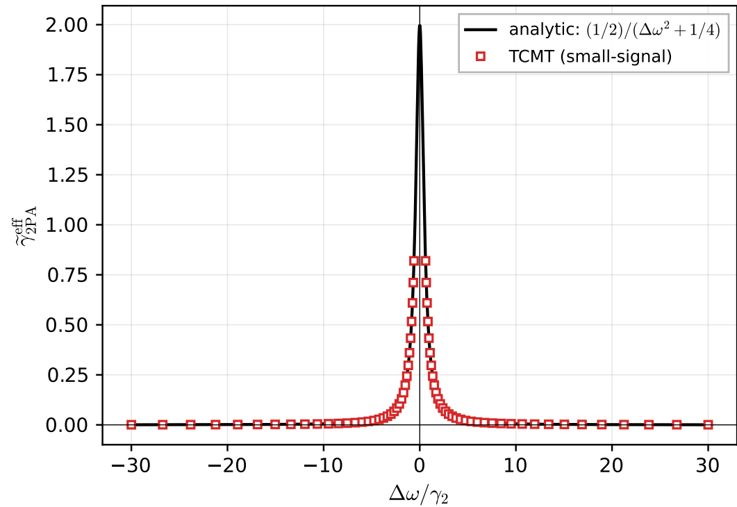
(b) Cascaded two-photon-like loss — Lorentzian, peak at \Delta\omega=0
