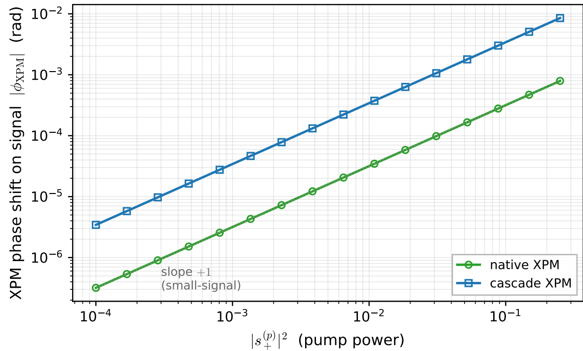
(a) XPM phase shift: cascade exceeds native by \sim(1+R)
