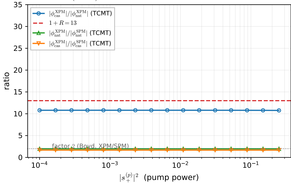
(b) (1+R) cascade/native and factor-2 XPM/SPM
