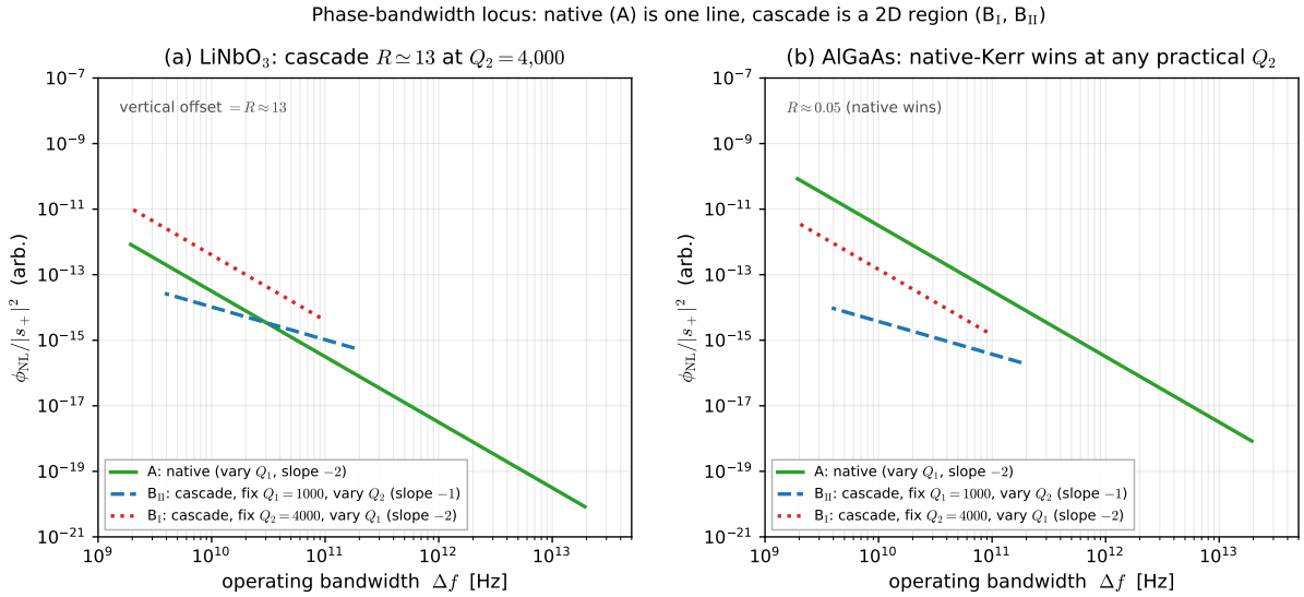
Figure 15. Per-photon nonlinear phase shift versus operating bandwidth on log-log. Native (A, green solid, slope -2) is a single line. Cascade is a 2-D region bounded by B_I (red dotted, slope -2, parallel to A but vertically offset by R ) and B_{II} (blue dashed, slope -1, the sum-rule line). (a) LiNbO 3 : R \approx 13 , cascade wins across the plotted range. (b) AlGaAs: R \approx 0.05 , native wins.
