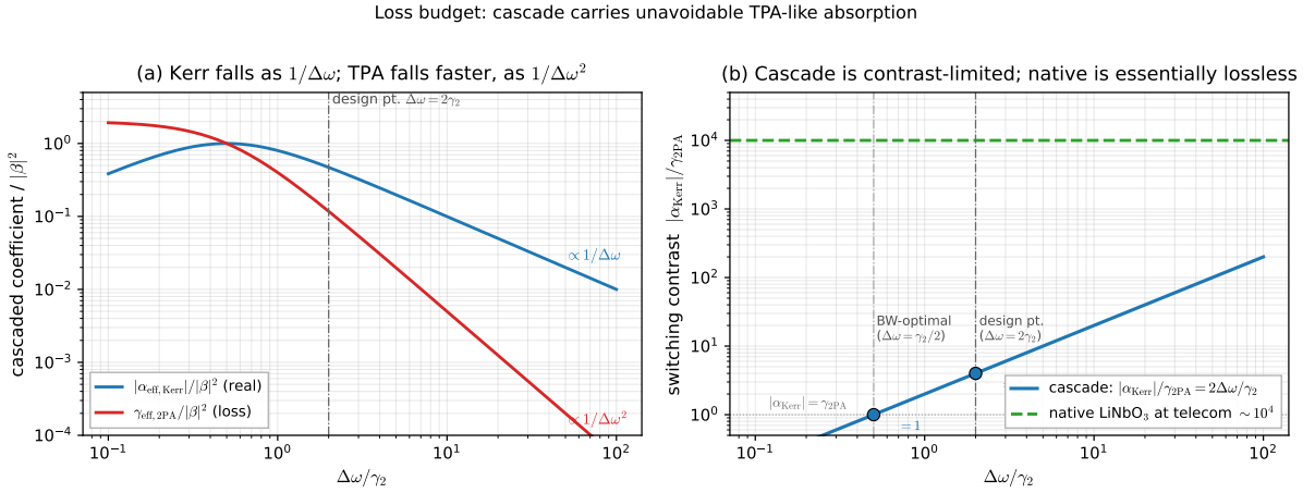
Figure 17. (a) Real (Kerr) and imaginary (TPA) parts of the cascaded coefficient vs. \Delta\omega/\gamma_2 . Kerr falls as 1/\Delta\omega (far-detuned); TPA falls faster, as 1/\Delta\omega^2 , so contrast (Kerr/TPA) grows linearly with \Delta\omega . (b) Cascade switching contrast = 2\Delta\omega/\gamma_2 vs. \Delta\omega/\gamma_2 , compared with the native LiNbO 3 contrast at telecom ( \sim 10^4 , set by residual material absorption).
