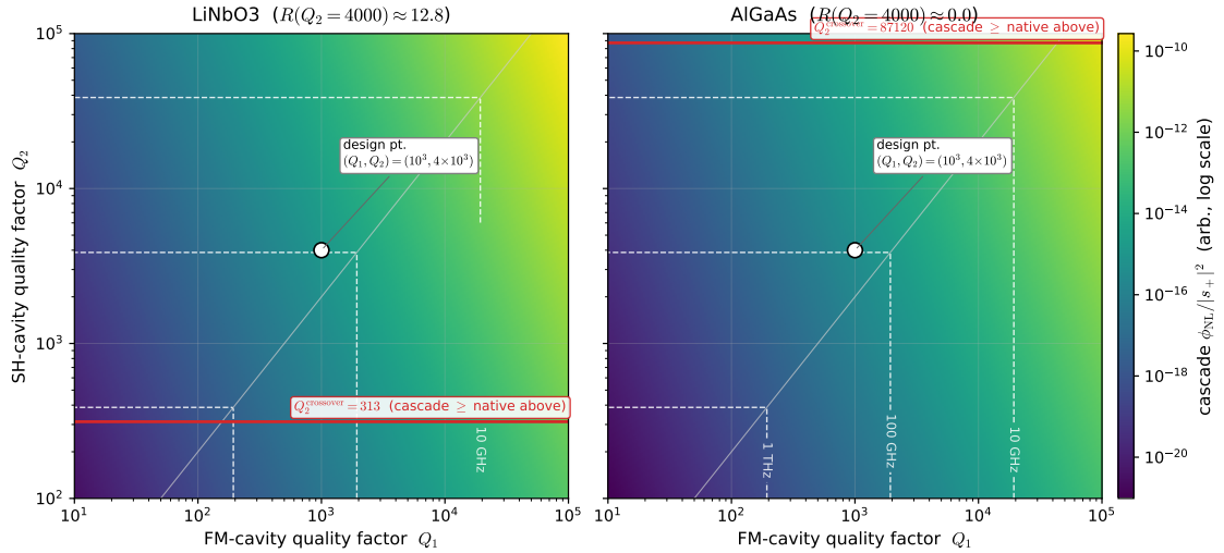
Figure 16. Cascade \phi_{\text{NL}}/|s_+|^2 on the (Q_1, Q_2) plane, shared colour scale across panels. White dashed contours: operating bandwidth \Delta f = \min(\gamma_1, \gamma_2)/(2\pi) . Red horizontal: Q_2 = Q_2^{\text{crossover}} (cascade \geq native above). Grey diagonal: Q_1 = Q_2/2 (FM-bottleneck \leftrightarrow SH-bottleneck boundary). White marker: design point (Q_1, Q_2) = (10^3, 4 \times 10^3) .
