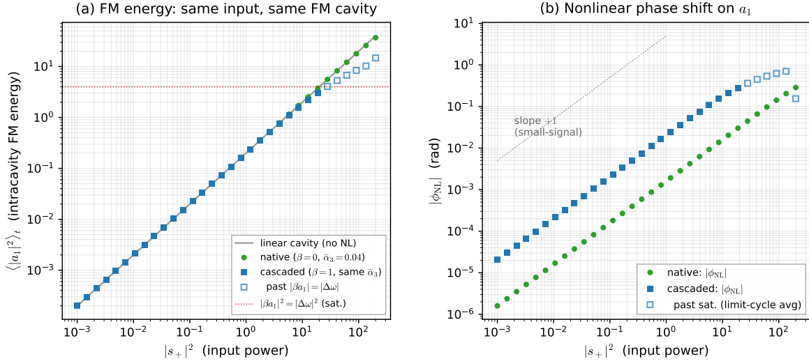
Figure 13. Direct TCMT comparison of the two architectures under identical CW input and identical FM cavity. (a) Intracavity FM energy |a_1|^2 vs. input power: native sits on the linear-cavity reference (its tiny bare Kerr barely deflects it); cascade peels below and saturates at |a_1|^2 \rightarrow |\Delta\omega|^2 . (b) Magnitudes of the nonlinear phase shift on a_1 . At small signal, the cascade phase is \sim 12\times larger than the native phase, matching the predicted ratio R = 12 (LiNbO 3 conservative operating point, \Delta\omega = 2\gamma_2 , factor-24 prefactor) within a few percent.
