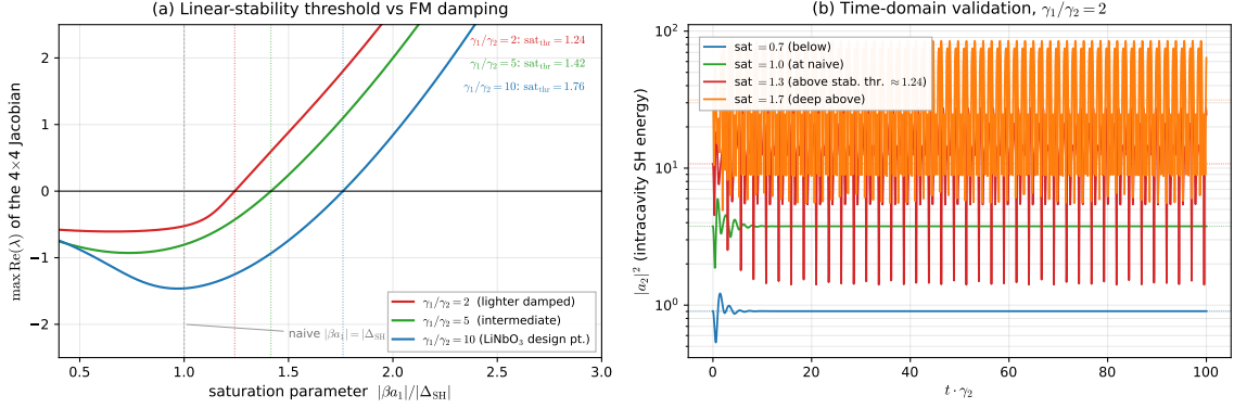
Figure 6. (a) Largest real part of the 4 \times 4 Jacobian eigenvalue of the trivial fixed point versus the saturation parameter, for three FM-damping levels. The crossing of zero is the parametric-oscillation threshold: \text{sat}_{\text{thr}} = 1.24, 1.42, 1.76 for \gamma_1/\gamma_2 = 2, 5, 10 respectively. The realistic LiNbO 3 design point ( \gamma_1/\gamma_2 = 10 ) sits at \text{sat}_{\text{thr}} \approx 1.76 , well above the naive |\beta a_1| = |\Delta_{\text{SH}}| mark. (b) Time-domain validation at the lighter-damped \gamma_1/\gamma_2 = 2 , chosen so the threshold sits at numerically tractable input. Below threshold, a 10^{-3} SH perturbation decays back to the trivial FP; above threshold, the trajectory enters a clear limit cycle. Dotted lines show the trivial-FP values of matching colour.
