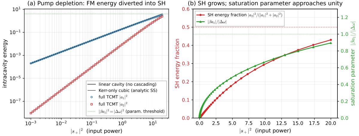
Figure 5. (a) Log–log of intracavity energies. Linear-cavity reference (grey), Kerr-only cubic (black), full TCMT with cascading (open markers). The cubic and the TCMT trivial fixed point are equivalent to machine precision. (b) Linear-x view: SH energy fraction (red, left) and saturation parameter |\beta a_1|/|\Delta\omega| (green, right) climb together.
