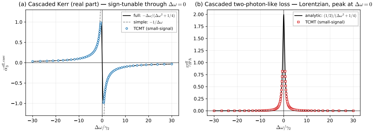
Figure 1. Cascaded effective coefficients extracted from steady-state TCMT (open markers) compared with closed-form analytic curves (black solid). (a) real (Kerr) part; (b) imaginary (two-photon-like loss) part.
