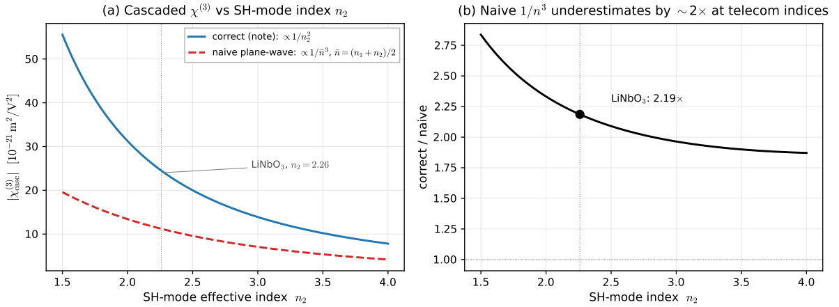
Figure 11. (a) |\chi_{\text{casc}}^{(3)}| versus SH-mode index n_2 at fixed Q_2 = 4000 , \eta_{\text{geom}} = 0.3 . The resonant single-mode result (5) (blue) versus the bulk plane-wave 1/\bar{n}^3 form (red, with \bar{n} = (n_1 + n_2)/2 ). (b) Their ratio. At LiNbO 3 ( n_2 = 2.26 ) the ratio is 2.19, matching \bar{n}^3/n_2^2 = 2.18 . The figure is comparing two derivations side-by-side, not validating one against the other: the bulk form is incorrect for resonant single-mode cascading because the four powers of n_1 do not appear in the bulk derivation.
