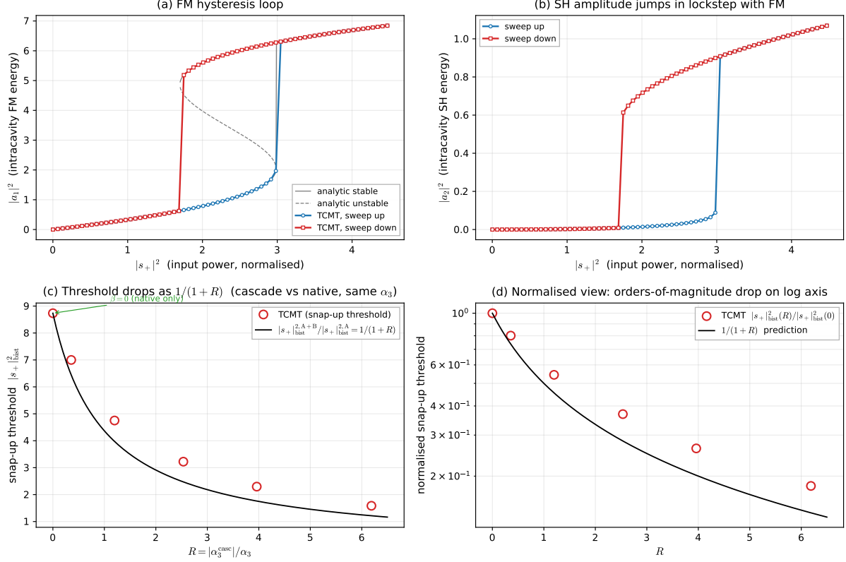
Figure 4. (a) Hysteresis in the intracavity FM energy under a stepwise quasi-static input sweep. The pump is detuned blue of the cold-cavity resonance ( \delta_p > 0 ) so that the intensity-induced red-shift of the dressed FM resonance (negative cascaded Kerr at \Delta\omega > 0 ) climbs toward the pump as input grows – the standard geometry for self-defocusing-Kerr bistability. Snap-up at |s_+|^2 \approx 3.0 , snap-down at \approx 1.7 ; both sit on the analytic Kerr+2PA saddle-nodes. (b) SH amplitude jumps in lockstep with the FM, tied by a_2 = i\beta a_1^2/(\gamma_2/2 - i\Delta_{\text{SH}}) . (c,d) Threshold-vs- R sweep at fixed \Delta\omega , \delta_p , and \alpha_3 (constructive sign): native Kerr ( \beta = 0 ) anchors R = 0 ; increasing \beta adds an aligned cascade contribution \alpha_3^{\text{casc}} , raising R . TCMT measurements (red) follow the predicted 1/(1+R) scaling (black) to within \sim 30\% ; the residual is the cascaded TPA-driven cusp distortion that the pure-Kerr 1/(1+R) formula does not capture.
