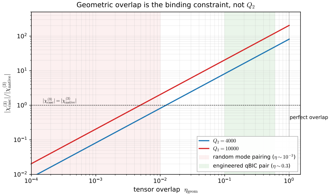
Figure 10. Cascaded enhancement versus tensor overlap \eta_{\text{geom}} on log-log, for two Q_2 values. Random mode pairing ( \eta_{\text{geom}} \sim 10^{-3} , red shaded) gives sub-native cascading even at Q_2 = 10^4 . Engineered qBIC pair ( \eta_{\text{geom}} \sim 0.3 , green shaded) recovers 25\text{--}60 \times enhancement.
