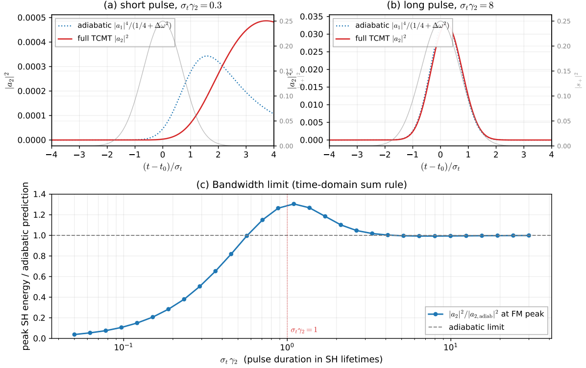
Figure 7. (a) Short pulse \sigma_t \gamma_2 = 0.3 : the SH lags and undershoots the adiabatic prediction (blue dotted), then rings down at rate \gamma_2/2 . (b) Long pulse \sigma_t \gamma_2 = 8 : the SH faithfully tracks |a_1|^2 . (c) Tracking quality at the moment of FM peak across \sigma_t \gamma_2 \in [0.05, 30] . The ratio crosses unity at \sigma_t \gamma_2 \approx 1 – the time-domain face of the bandwidth–enhancement sum rule – and overshoots to \sim 1.3 near \sigma_t \gamma_2 = 1 before settling. The overshoot is not numerical ringing: at marginal pulse duration the FM peaks just before the SH catches up, and the SH receives a brief impulsive drive that pushes its peak above the static adiabatic value |a_1|^4 / (\Delta\omega^2 + (\gamma_2/2)^2) for an instant.
