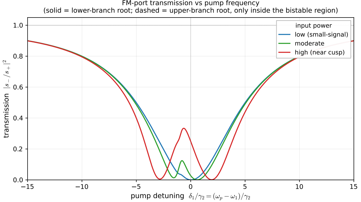
Figure 12. FM-port transmission |s_-/s_+|^2 versus pump detuning \delta_p/\gamma_2 at three input powers. The low-power curve is a clean critically-coupled Lorentzian dip; the high-power curve shows the lineshape distortion through cascaded Kerr self-detuning combined with the sign flip of \alpha_3^{\text{eff,casc}} as \Delta_{\text{SH}} crosses zero, producing the characteristic double-dip pattern unique to a doubly-resonant cascaded system.
