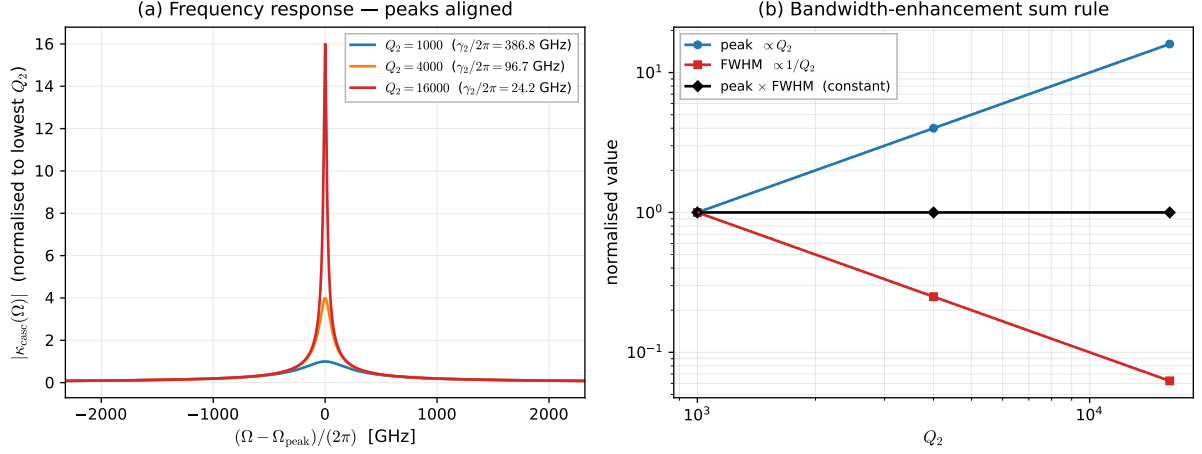
Figure 3. (a) Modulation transfer function |\kappa_{\text{casc}}(\Omega)| evaluated on a shared \Omega grid for three Q_2 values, peaks aligned at \Omega = -\Delta_{\text{SH}} . (b) Peak grows \propto Q_2 ; FWHM shrinks \propto 1/Q_2 ; their product is Q_2 -independent.
