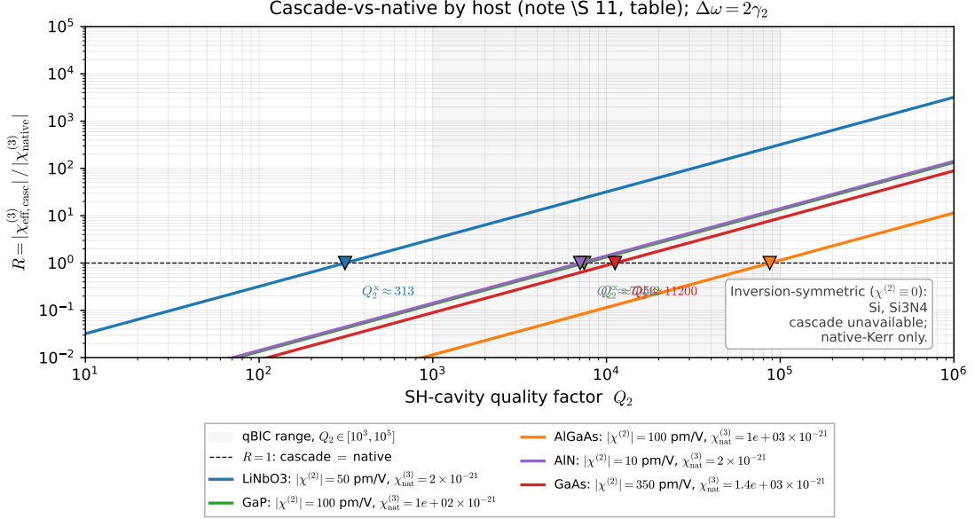
Figure 14. Cascaded enhancement ratio R(Q_2) for five non-centrosymmetric hosts, log–log. Native sits on the dashed line at R = 1 . Crossover markers ( \nabla ) indicate Q_2^{\text{crossover}} at which R = 1 for each host. Inversion-symmetric hosts (Si, \text{Si}_3\text{N}_4 ) have no cascade route: \chi^{(2)} \equiv 0 .
