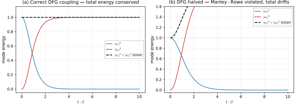
Figure 8. Lossless TCMT, no input. (a) Correct DFG factor: total energy stays at 1.0 to machine precision. (b) Halved DFG (the “ \kappa vs \kappa/2 ” bug of the original derivation): total energy grows past 1.6 by t = 2/\beta – energy created out of nothing.
