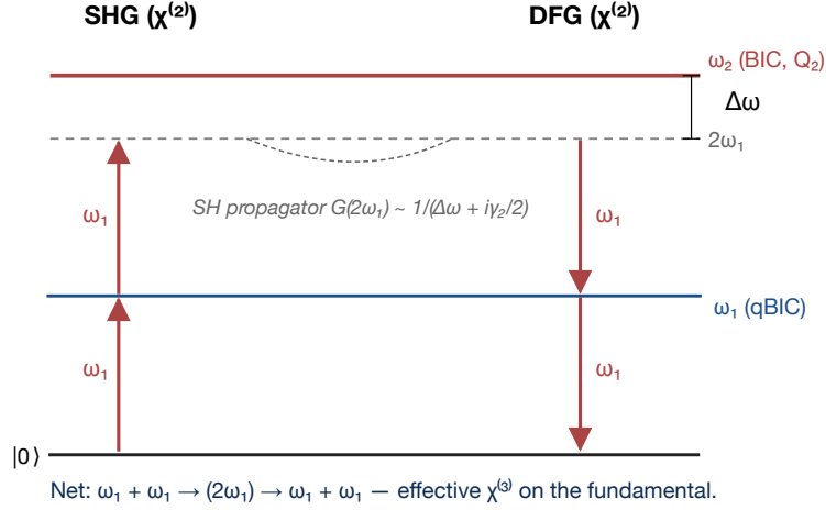
Figure 1: Energy-level diagram of the cascade. SHG (up arrows) virtually populates the SH level at 2\omega_1 off-resonant from the BIC at \omega_2 by \Delta\omega = 2\omega_1 - \omega_2 ; DFG (down arrows) returns to two \omega_1 photons. The SH propagator G(2\omega_1) \sim 1/(\Delta\omega + i\gamma_2/2) controls the strength of the cascade.
