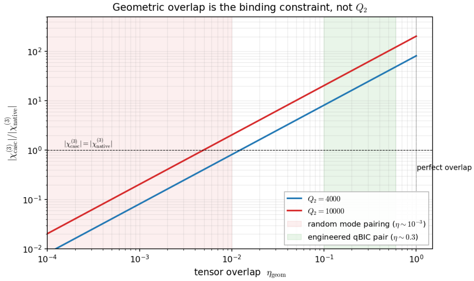
Figure 15: \eta_{\text{geom}} spans three orders of magnitude — random mode pairings give \eta \sim 10^{-3} ; engineered qBIC pairs reach \eta \sim 0.3 . The cascade ratio R scales linearly with \eta^{**} .
