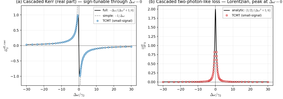
Figure 3: Full-TCMT \phi_{\text{NL}}/|s_+|^2 vs analytic 8\alpha_3^{\text{eff}}/\gamma_1^2 as \Delta\omega is swept (numerical self-consistency check at small signal).
