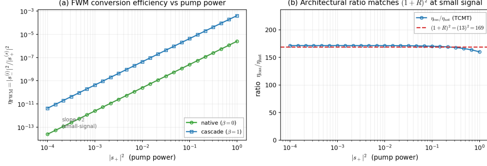
Figure 7: TCMT FWM efficiency: cascade outperforms native by (1 + R)^2 = 169 at small signal (numerical self-consistency check).
