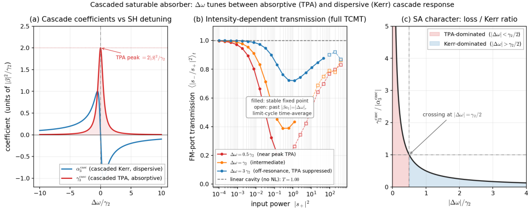
Figure 2: Cascade Kerr (blue, S-shaped) and TPA (red, Lorentzian) coefficients vs SH detuning. Loss/Kerr ratio crosses 1 at |\Delta\omega| = \gamma_2/2 .
