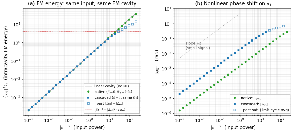
Figure 5: Constructive cascade ( \Delta\omega = -2\gamma_2 ) gives the small-signal phase ratio \simeq 1 + R \simeq 13 , matching TCMT to within 1 %.
