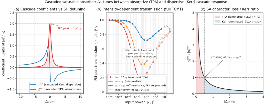
Figure 10: SA: dispersive Kerr (blue, S-curve) and absorptive TPA (red, Lorentzian peak). Intensity-dependent transmission (panel b) pulls T from 1 toward critical coupling. Crossover at |\Delta\omega| = \gamma_2/2 .
