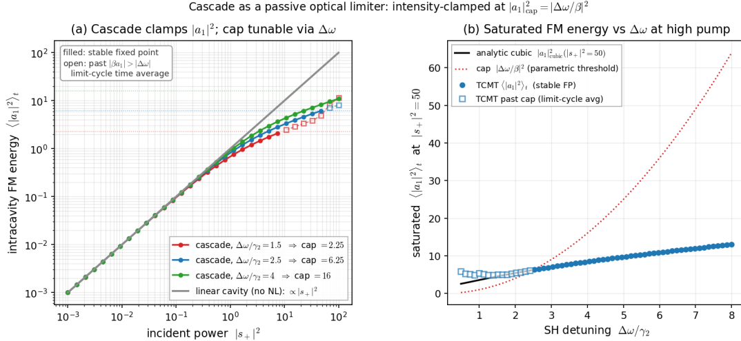
Figure 12: (a) Full-TCMT |a_1|^2 vs pump for three \Delta\omega values: cascade clamps at |\Delta\omega|^2 . (b) Saturated |a_1|^2 vs \Delta\omega : black cubic = correct prediction below threshold; red dotted = |\Delta\omega|^2 asymptote.
