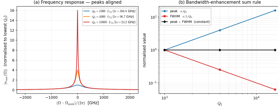
Figure 4: Sum-rule constancy: peak |\alpha_3^{\text{eff}}| \times \text{FWHM} is conserved across the Lorentzian. Note \text{FWHM}(|\alpha|) = \sqrt{3}\gamma_2 (broader), \text{FWHM}(|\alpha|^2) = \gamma_2 (proper Lorentzian); peak |\alpha| \times \text{FWHM}(|\alpha|) = 2\sqrt{3}|\beta|^2 .
