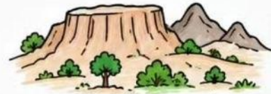
Old land, ancient rivers
